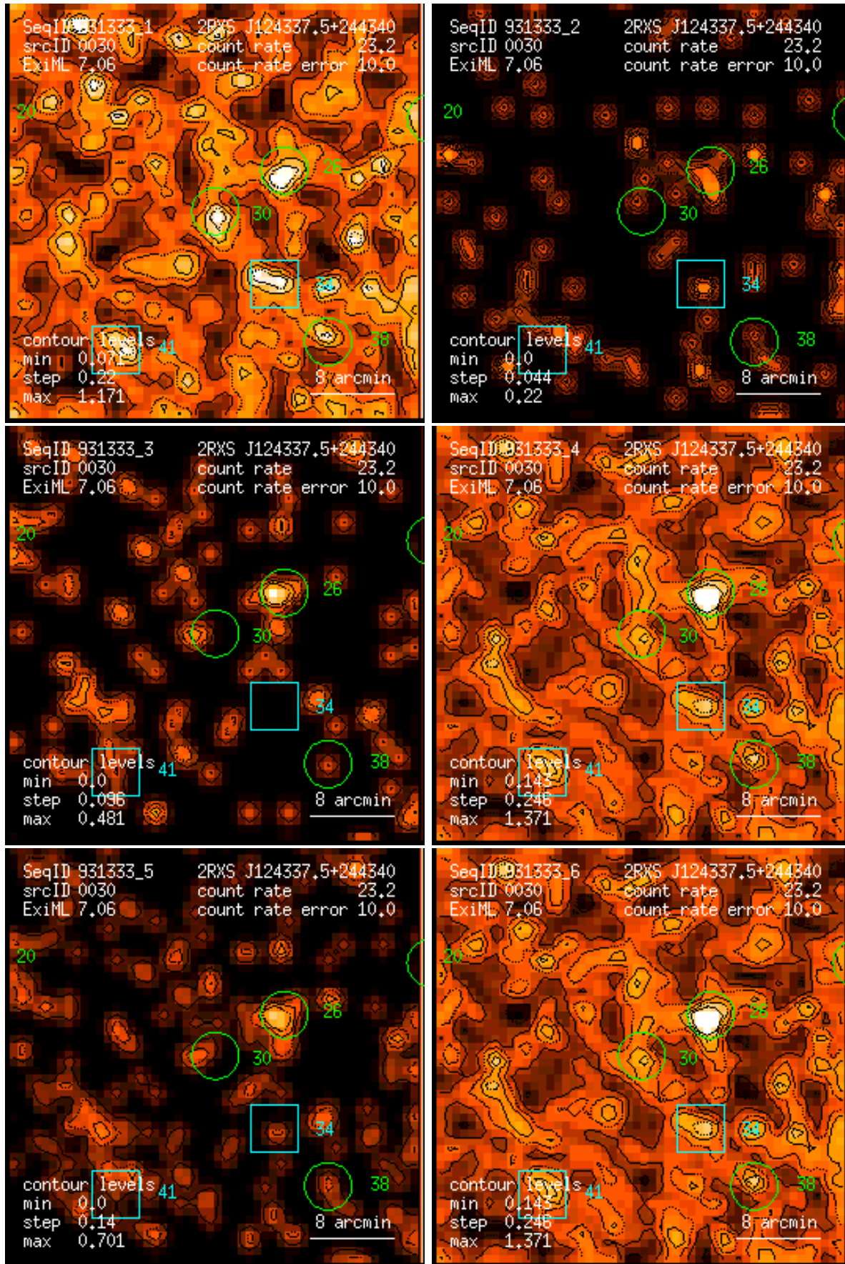
Figure 30: RASS 931333: detection 0030: band rate images, Gaussian filter: (1) PSPC channels 11 – 41, (2) 52 – 90, (3) 91 – 201, (4) 11 – 235, (5) 52 – 201, (6) 11 – 201. Broad band rates in counts/ks. Band rate contour levels in counts/ks/arcmin 2 .
