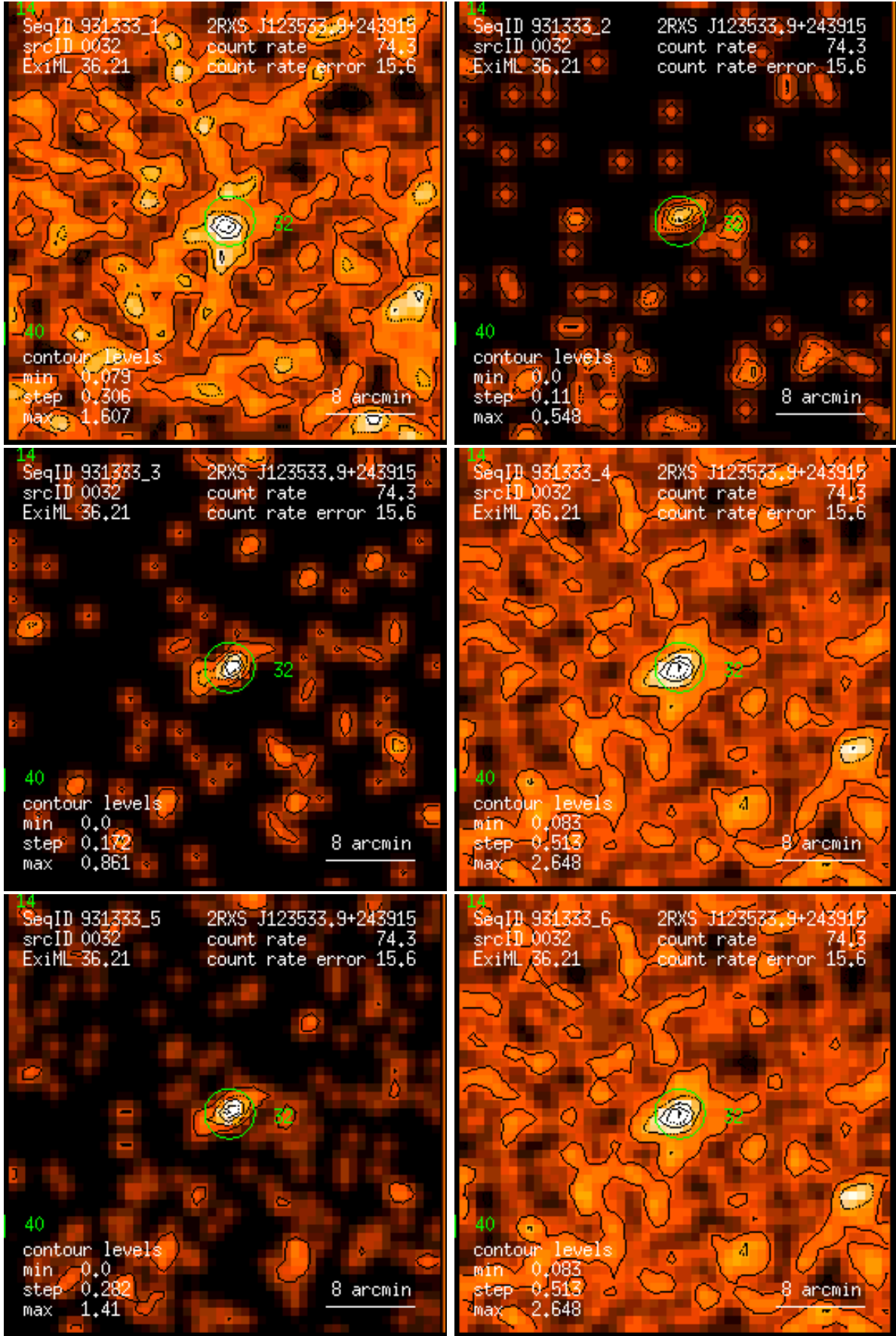
Figure 32: RASS 931333: detection 0032: band rate images, Gaussian filter: (1) PSPC channels 11 – 41, (2) 52 – 90, (3) 91 – 201, (4) 11 – 235, (5) 52 – 201, (6) 11 – 201. Broad band rates in counts/ks. Band rate contour levels in counts/ks/arcmin 2 .
