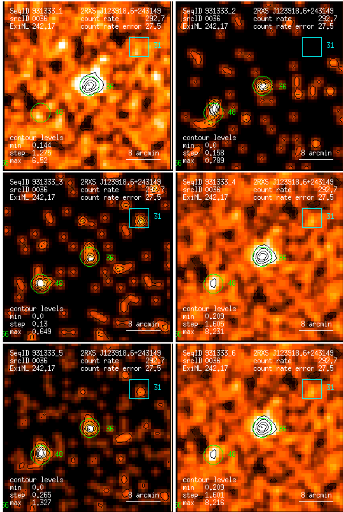
Figure 36: RASS 931333: detection 0036: band rate images, Gaussian filter: (1) PSPC channels 11 – 41, (2) 52 – 90, (3) 91 – 201, (4) 11 – 235, (5) 52 – 201, (6) 11 – 201. Broad band rates in counts/ks. Band rate contour levels in counts/ks/arcmin 2 .
