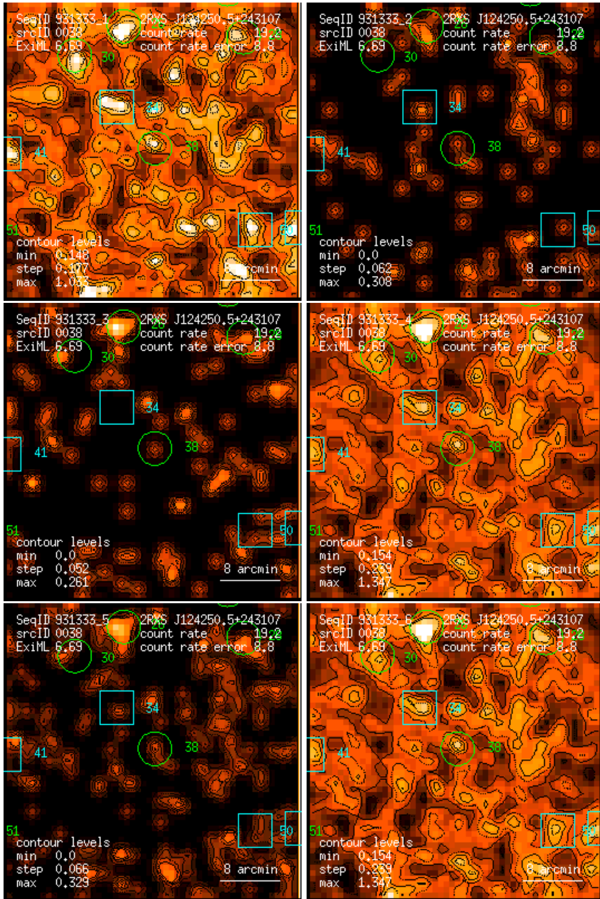
Figure 38: RASS 931333: detection 0038: band rate images, Gaussian filter: (1) PSPC channels 11 – 41, (2) 52 – 90, (3) 91 – 201, (4) 11 – 235, (5) 52 – 201, (6) 11 – 201. Broad band rates in counts/ks. Band rate contour levels in counts/ks/arcmin 2 .
