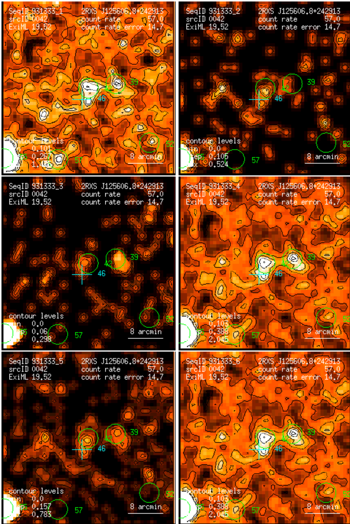
Figure 42: RASS 931333: detection 0042: band rate images, Gaussian filter: (1) PSPC channels 11 – 41, (2) 52 – 90, (3) 91 – 201, (4) 11 – 235, (5) 52 – 201, (6) 11 – 201. Broad band rates in counts/ks. Band rate contour levels in counts/ks/arcmin 2 .
