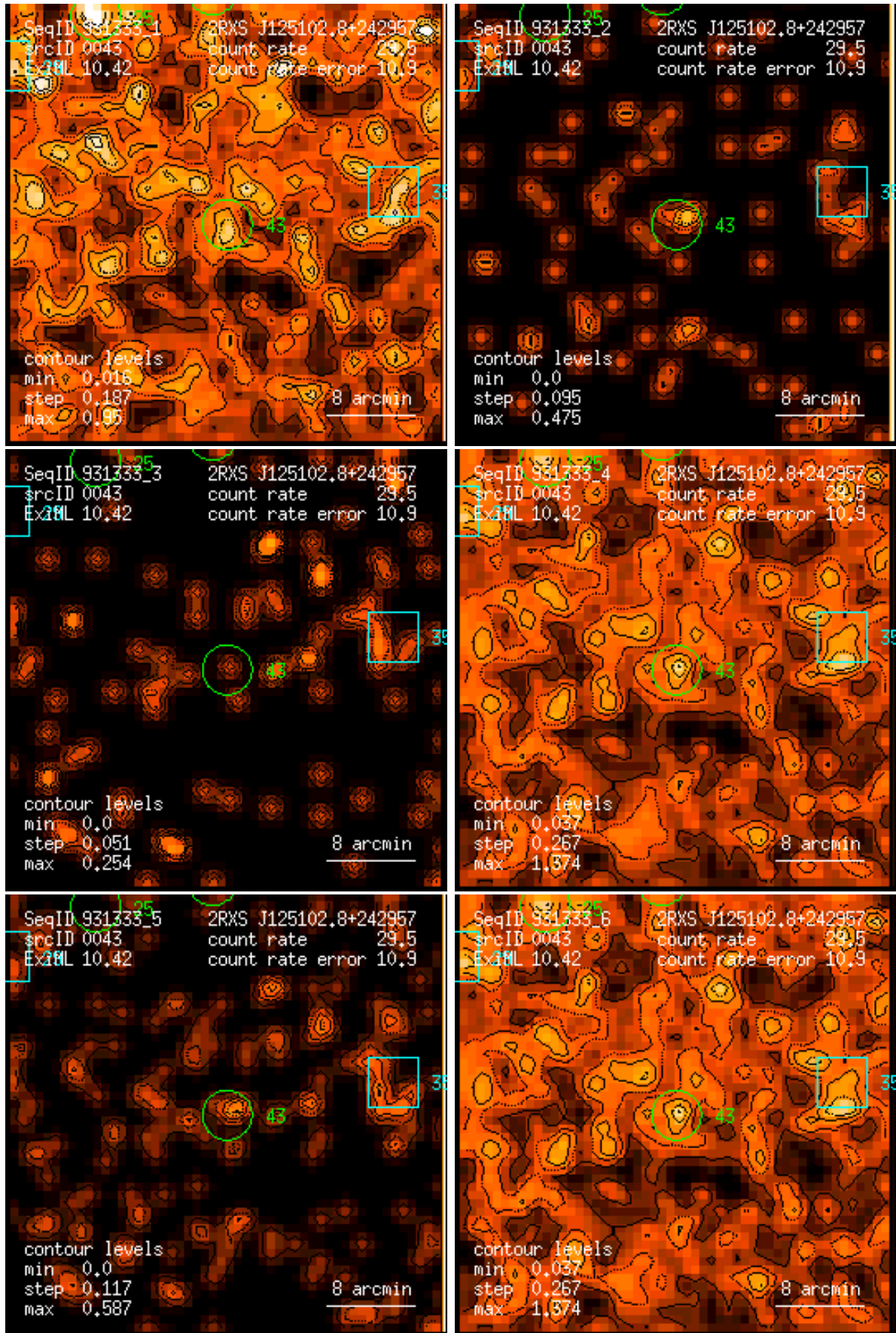
Figure 43: RASS 931333: detection 0043: band rate images, Gaussian filter: (1) PSPC channels 11 – 41, (2) 52 – 90, (3) 91 – 201, (4) 11 – 235, (5) 52 – 201, (6) 11 – 201. Broad band rates in counts/ks. Band rate contour levels in counts/ks/arcmin 2 .
