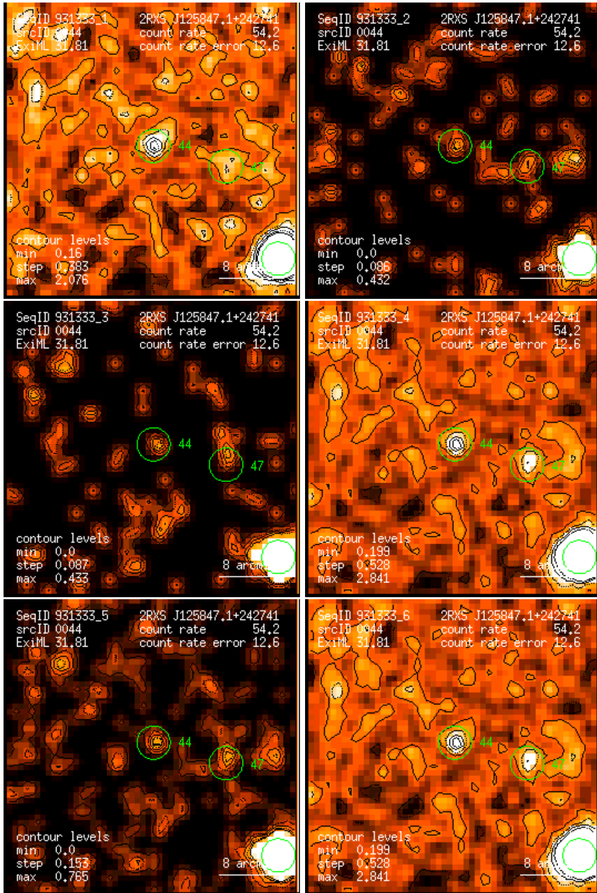
Figure 44: RASS 931333: detection 0044: band rate images, Gaussian filter: (1) PSPC channels 11 – 41, (2) 52 – 90, (3) 91 – 201, (4) 11 – 235, (5) 52 – 201, (6) 11 – 201. Broad band rates in counts/ks. Band rate contour levels in counts/ks/arcmin 2 .
