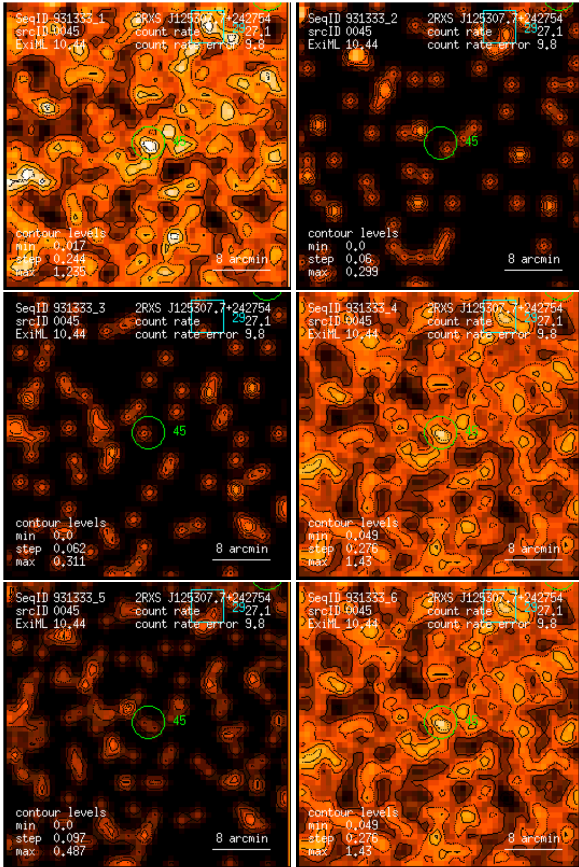
Figure 45: RASS 931333: detection 0045: band rate images, Gaussian filter: (1) PSPC channels 11 – 41, (2) 52 – 90, (3) 91 – 201, (4) 11 – 235, (5) 52 – 201, (6) 11 – 201. Broad band rates in counts/ks. Band rate contour levels in counts/ks/arcmin 2 .
