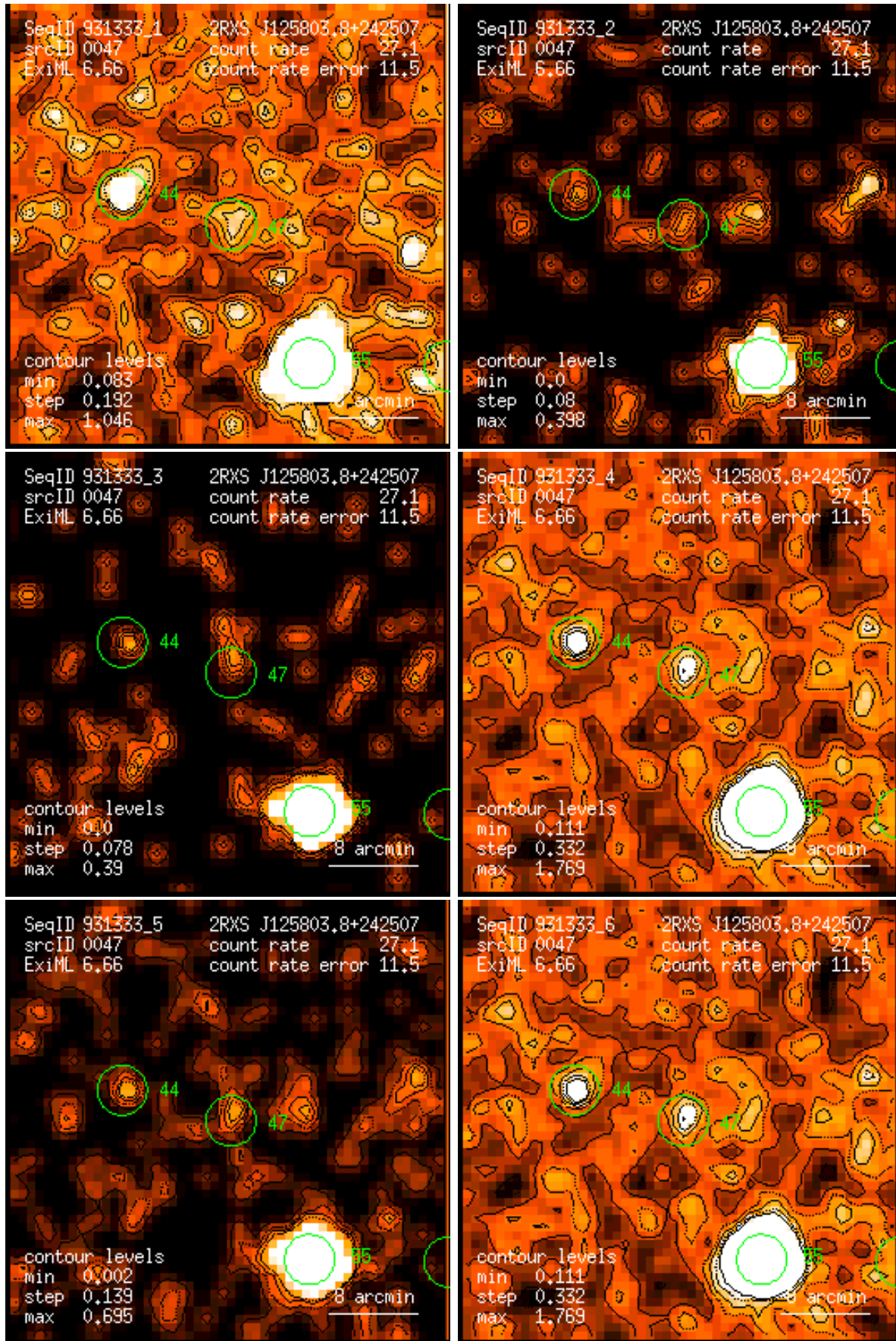
Figure 47: RASS 931333: detection 0047: band rate images, Gaussian filter: (1) PSPC channels 11 – 41, (2) 52 – 90, (3) 91 – 201, (4) 11 – 235, (5) 52 – 201, (6) 11 – 201. Broad band rates in counts/ks. Band rate contour levels in counts/ks/arcmin 2 .
