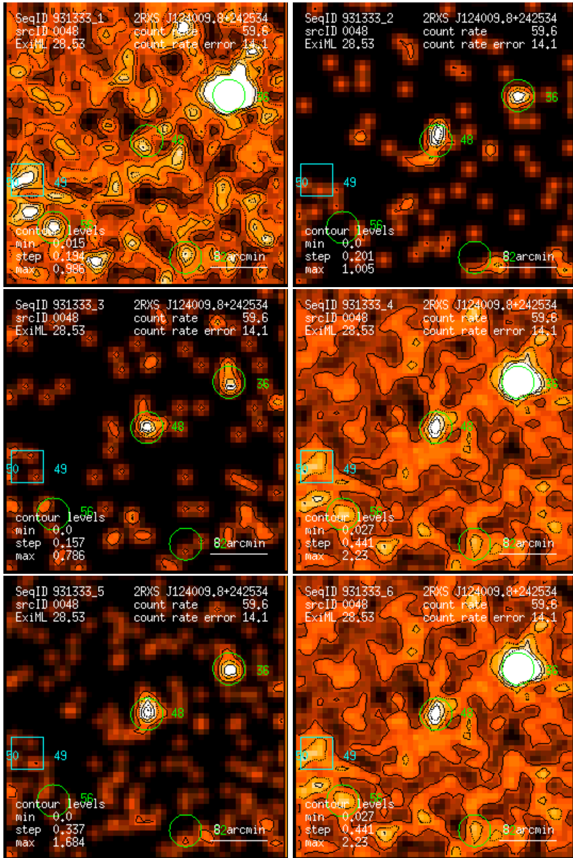
Figure 48: RASS 931333: detection 0048: band rate images, Gaussian filter: (1) PSPC channels 11 – 41, (2) 52 – 90, (3) 91 – 201, (4) 11 – 235, (5) 52 – 201, (6) 11 – 201. Broad band rates in counts/ks. Band rate contour levels in counts/ks/arcmin 2 .
