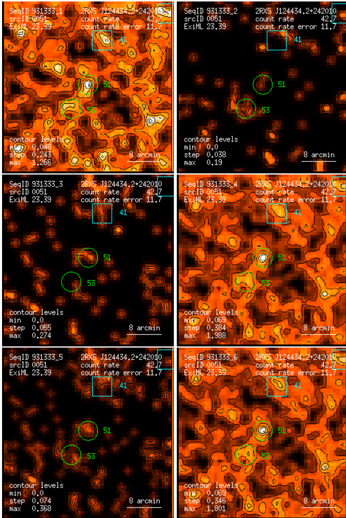
Figure 51: RASS 931333: detection 0051: band rate images, Gaussian filter: (1) PSPC channels 11 – 41, (2) 52 – 90, (3) 91 – 201, (4) 11 – 235, (5) 52 – 201, (6) 11 – 201. Broad band rates in counts/ks. Band rate contour levels in counts/ks/arcmin 2 .
