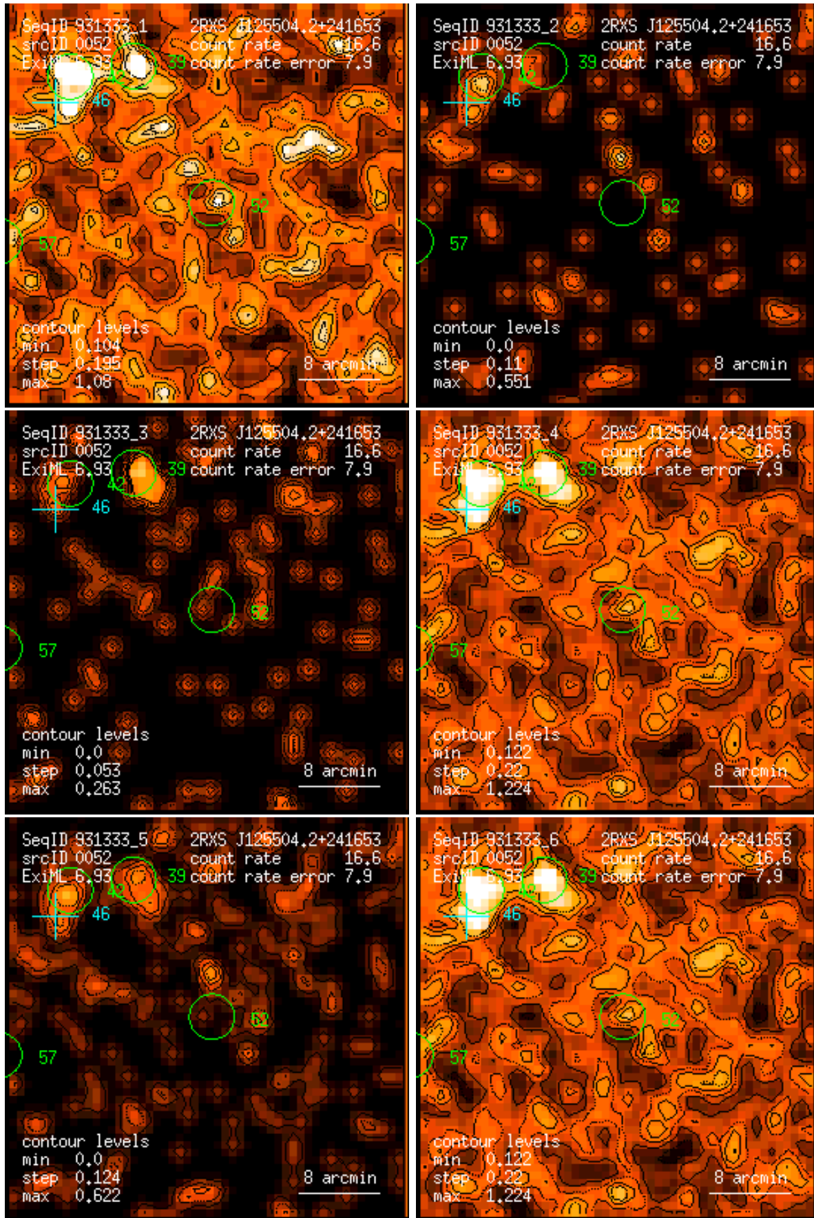
Figure 52: RASS 931333: detection 0052: band rate images, Gaussian filter: (1) PSPC channels 11 – 41, (2) 52 – 90, (3) 91 – 201, (4) 11 – 235, (5) 52 – 201, (6) 11 – 201. Broad band rates in counts/ks. Band rate contour levels in counts/ks/arcmin 2 .
