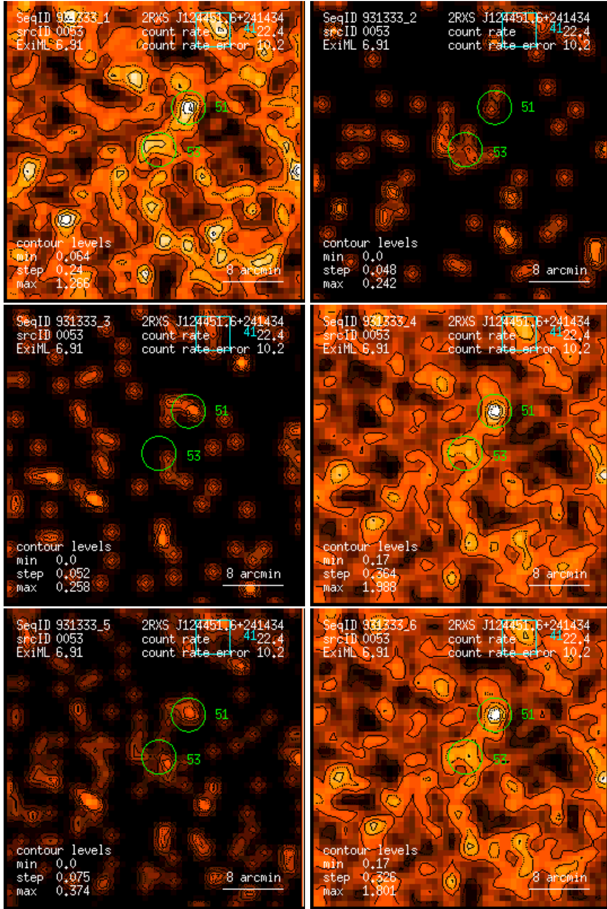
Figure 53: RASS 931333: detection 0053: band rate images, Gaussian filter: (1) PSPC channels 11 – 41, (2) 52 – 90, (3) 91 – 201, (4) 11 – 235, (5) 52 – 201, (6) 11 – 201. Broad band rates in counts/ks. Band rate contour levels in counts/ks/arcmin 2 .
