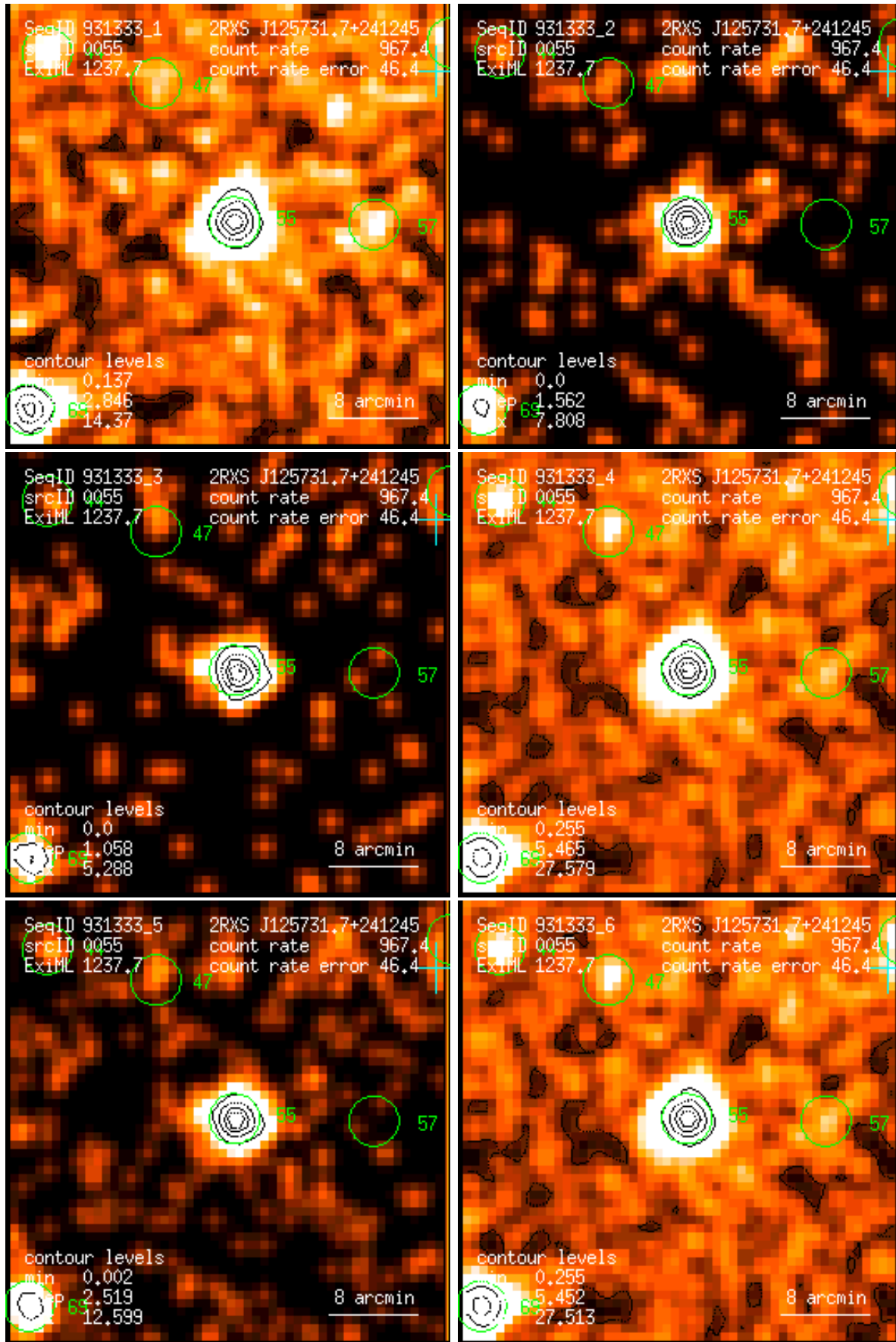
Figure 55: RASS 931333: detection 0055: band rate images, Gaussian filter: (1) PSPC channels 11 – 41, (2) 52 – 90, (3) 91 – 201, (4) 11 – 235, (5) 52 – 201, (6) 11 – 201. Broad band rates in counts/ks. Band rate contour levels in counts/ks/arcmin 2 .
