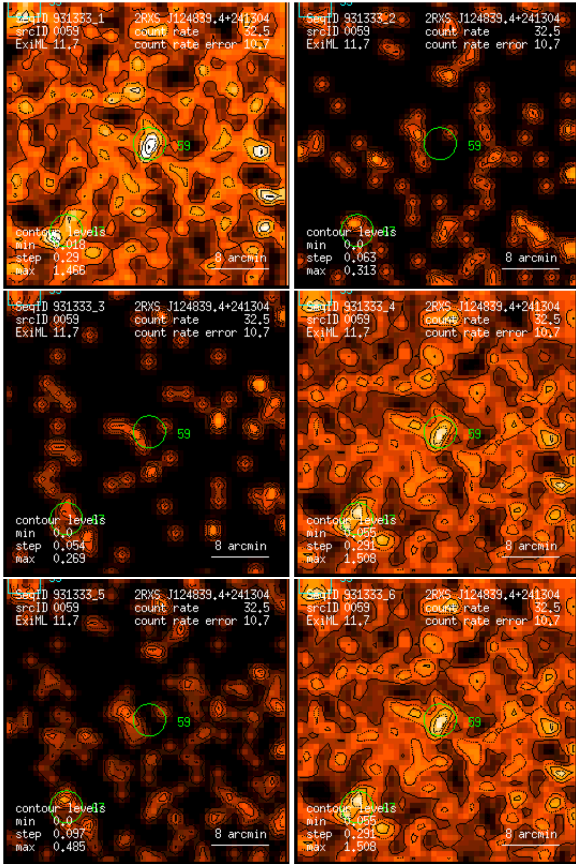
Figure 59: RASS 931333: detection 0059: band rate images, Gaussian filter: (1) PSPC channels 11 – 41, (2) 52 – 90, (3) 91 – 201, (4) 11 – 235, (5) 52 – 201, (6) 11 – 201. Broad band rates in counts/ks. Band rate contour levels in counts/ks/arcmin 2 .
