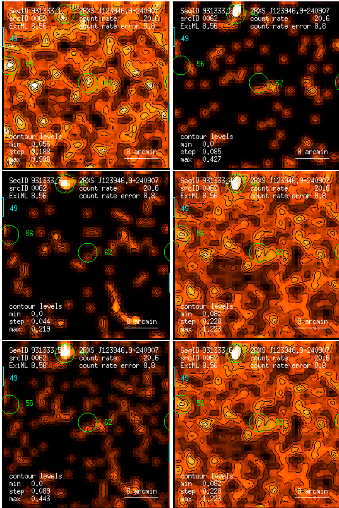
Figure 62: RASS 931333: detection 0062: band rate images, Gaussian filter: (1) PSPC channels 11 – 41, (2) 52 – 90, (3) 91 – 201, (4) 11 – 235, (5) 52 – 201, (6) 11 – 201. Broad band rates in counts/ks. Band rate contour levels in counts/ks/arcmin 2 .
