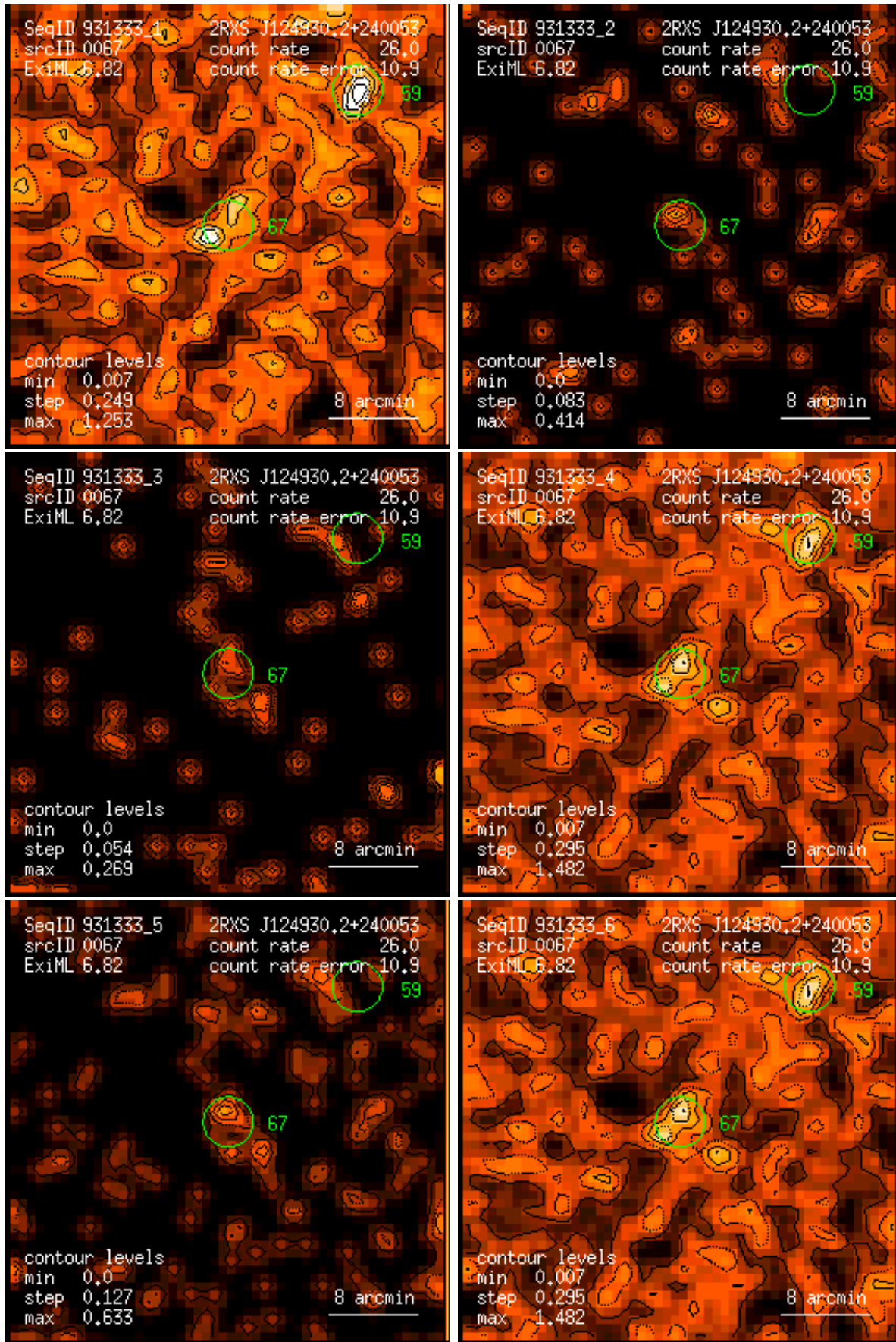
Figure 67: RASS 931333: detection 0067: band rate images, Gaussian filter: (1) PSPC channels 11 – 41, (2) 52 – 90, (3) 91 – 201, (4) 11 – 235, (5) 52 – 201, (6) 11 – 201. Broad band rates in counts/ks. Band rate contour levels in counts/ks/arcmin 2 .
