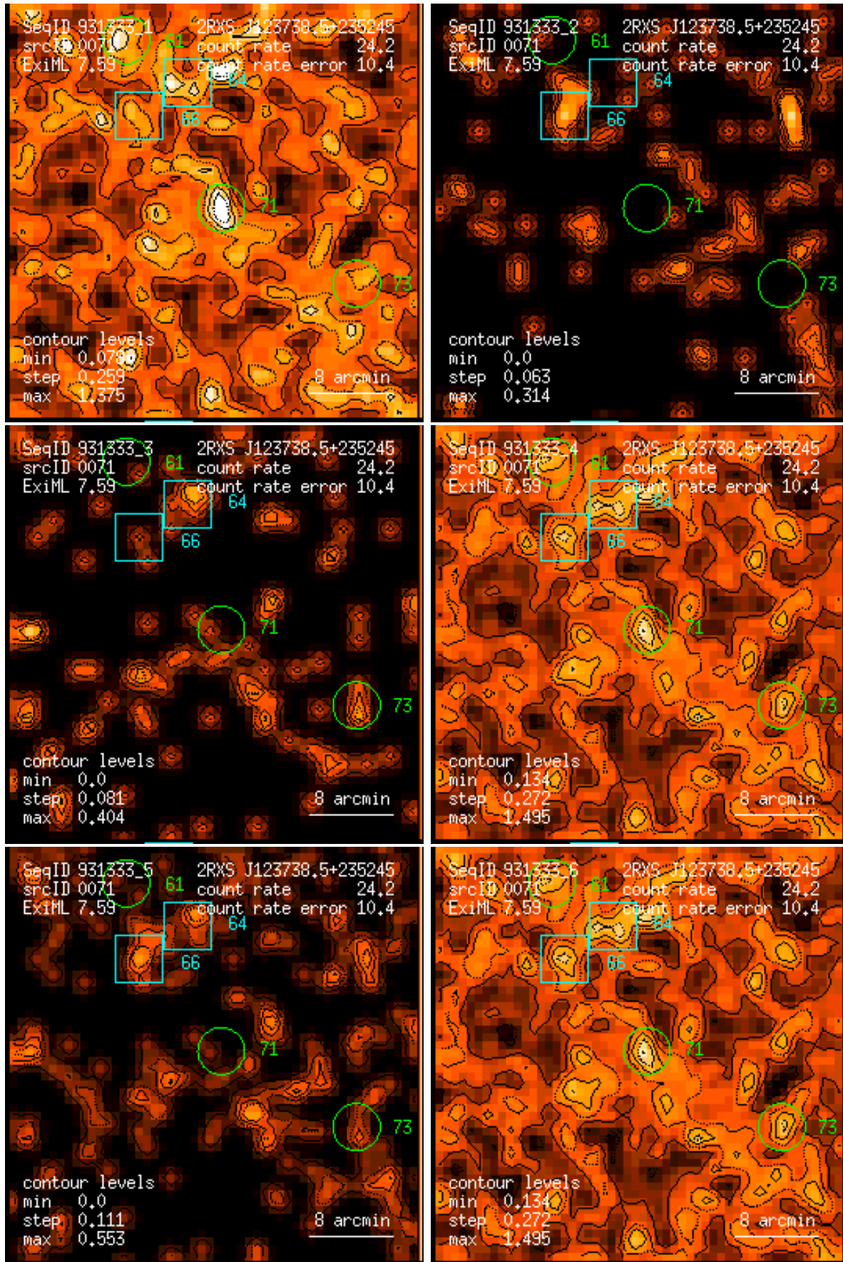
Figure 71: RASS 931333: detection 0071: band rate images, Gaussian filter: (1) PSPC channels 11 – 41, (2) 52 – 90, (3) 91 – 201, (4) 11 – 235, (5) 52 – 201, (6) 11 – 201. Broad band rates in counts/ks. Band rate contour levels in counts/ks/arcmin 2 .
