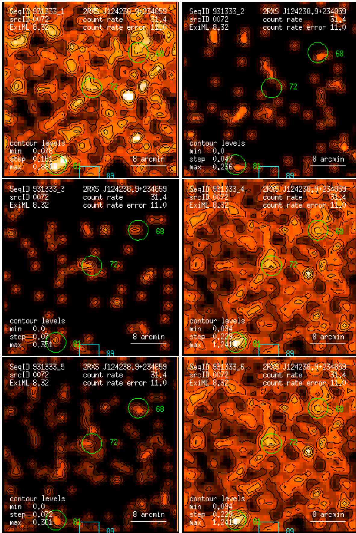
Figure 72: RASS 931333: detection 0072: band rate images, Gaussian filter: (1) PSPC channels 11 – 41, (2) 52 – 90, (3) 91 – 201, (4) 11 – 235, (5) 52 – 201, (6) 11 – 201. Broad band rates in counts/ks. Band rate contour levels in counts/ks/arcmin 2 .
