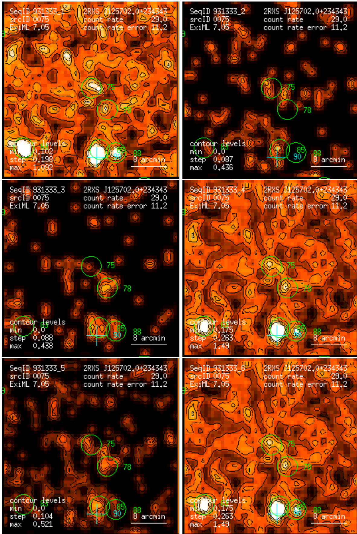
Figure 75: RASS 931333: detection 0075: band rate images, Gaussian filter: (1) PSPC channels 11 – 41, (2) 52 – 90, (3) 91 – 201, (4) 11 – 235, (5) 52 – 201, (6) 11 – 201. Broad band rates in counts/ks. Band rate contour levels in counts/ks/arcmin 2 .
