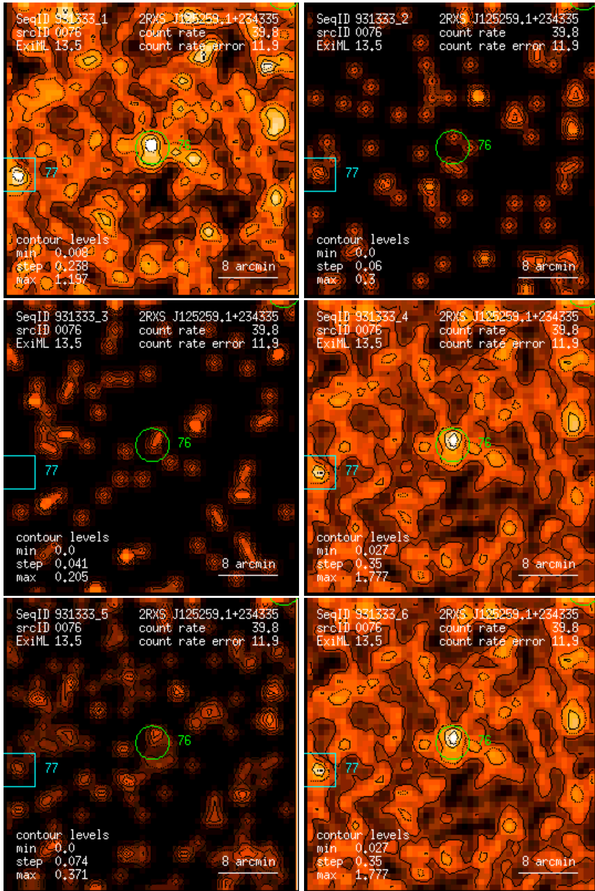
Figure 76: RASS 931333: detection 0076: band rate images, Gaussian filter: (1) PSPC channels 11 – 41, (2) 52 – 90, (3) 91 – 201, (4) 11 – 235, (5) 52 – 201, (6) 11 – 201. Broad band rates in counts/ks. Band rate contour levels in counts/ks/arcmin 2 .
