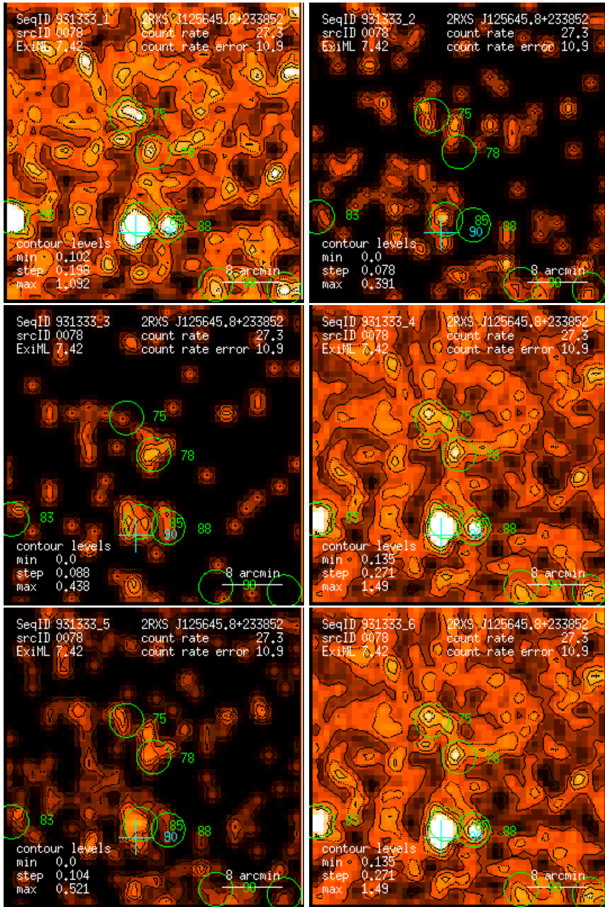
Figure 78: RASS 931333: detection 0078: band rate images, Gaussian filter: (1) PSPC channels 11 – 41, (2) 52 – 90, (3) 91 – 201, (4) 11 – 235, (5) 52 – 201, (6) 11 – 201. Broad band rates in counts/ks. Band rate contour levels in counts/ks/arcmin 2 .
