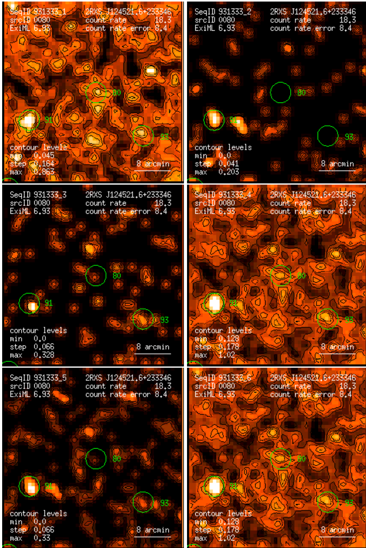
Figure 80: RASS 931333: detection 0080: band rate images, Gaussian filter: (1) PSPC channels 11 – 41, (2) 52 – 90, (3) 91 – 201, (4) 11 – 235, (5) 52 – 201, (6) 11 – 201. Broad band rates in counts/ks. Band rate contour levels in counts/ks/arcmin 2 .
