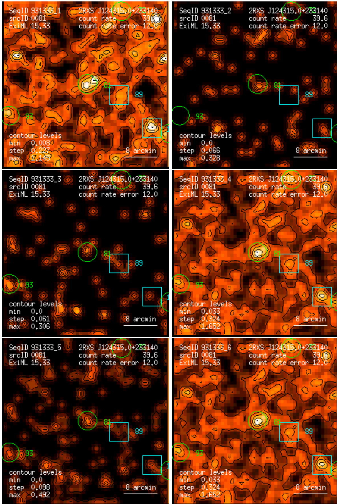
Figure 81: RASS 931333: detection 0081: band rate images, Gaussian filter: (1) PSPC channels 11 – 41, (2) 52 – 90, (3) 91 – 201, (4) 11 – 235, (5) 52 – 201, (6) 11 – 201. Broad band rates in counts/ks. Band rate contour levels in counts/ks/arcmin 2 .
