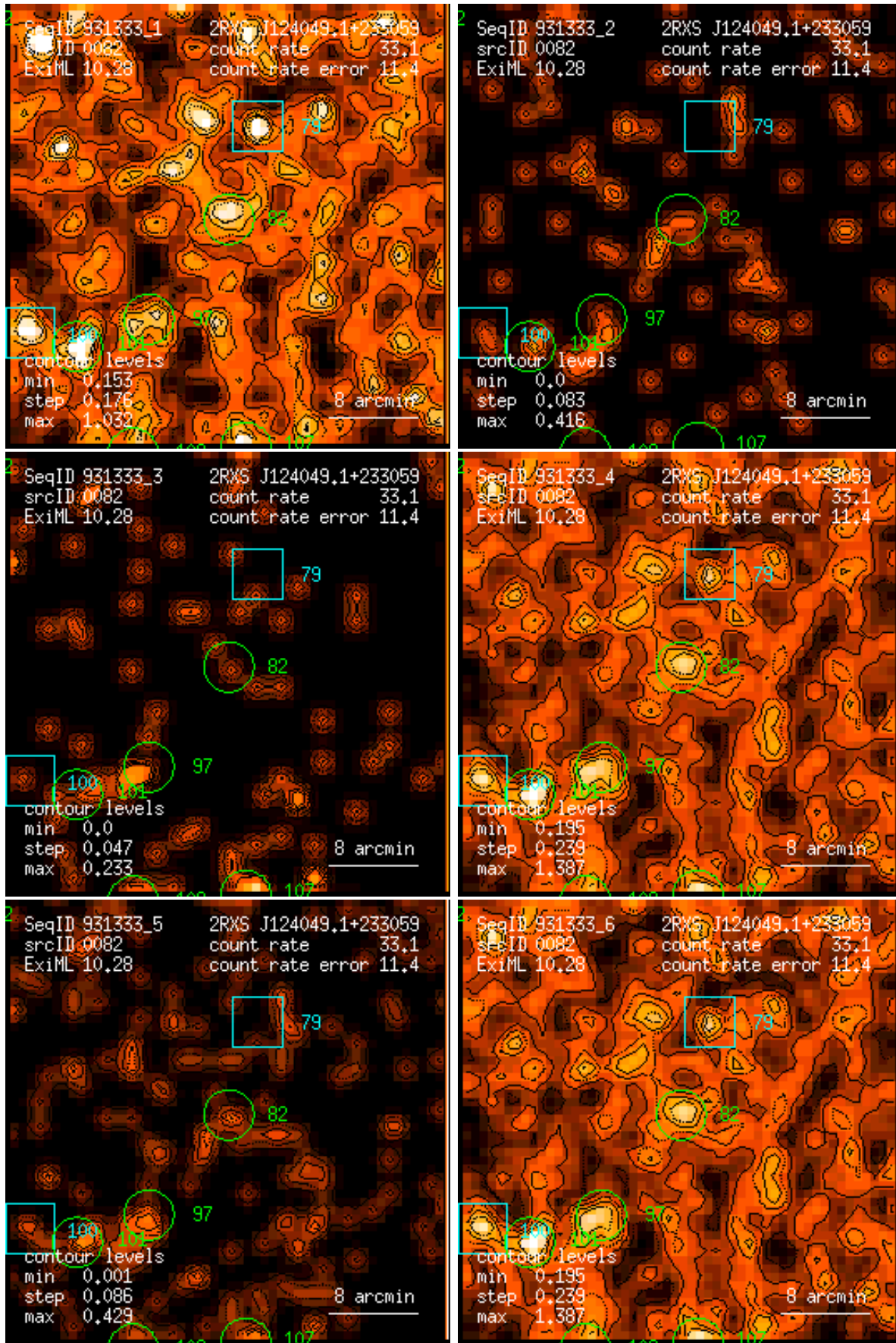
Figure 82: RASS 931333: detection 0082: band rate images, Gaussian filter: (1) PSPC channels 11 – 41, (2) 52 – 90, (3) 91 – 201, (4) 11 – 235, (5) 52 – 201, (6) 11 – 201. Broad band rates in counts/ks. Band rate contour levels in counts/ks/arcmin 2 .
