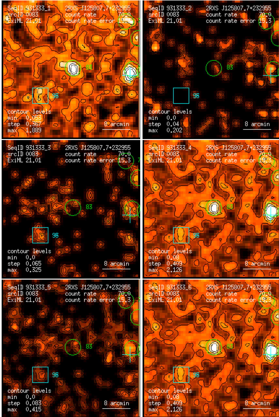
Figure 83: RASS 931333: detection 0083: band rate images, Gaussian filter: (1) PSPC channels 11 – 41, (2) 52 – 90, (3) 91 – 201, (4) 11 – 235, (5) 52 – 201, (6) 11 – 201. Broad band rates in counts/ks. Band rate contour levels in counts/ks/arcmin 2 .
