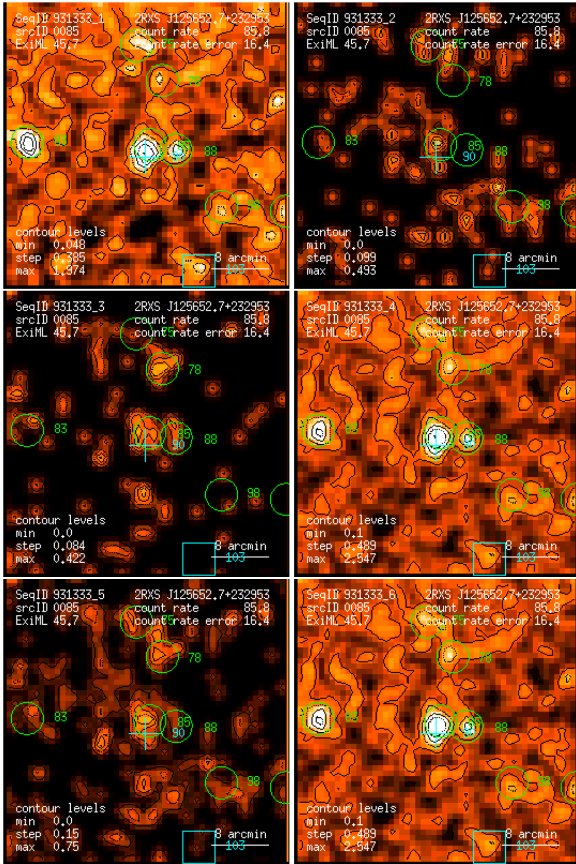
Figure 85: RASS 931333: detection 0085: band rate images, Gaussian filter: (1) PSPC channels 11 – 41, (2) 52 – 90, (3) 91 – 201, (4) 11 – 235, (5) 52 – 201, (6) 11 – 201. Broad band rates in counts/ks. Band rate contour levels in counts/ks/arcmin 2 .
