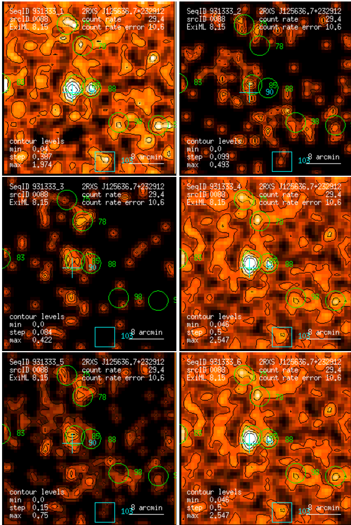
Figure 88: RASS 931333: detection 0088: band rate images, Gaussian filter: (1) PSPC channels 11 – 41, (2) 52 – 90, (3) 91 – 201, (4) 11 – 235, (5) 52 – 201, (6) 11 – 201. Broad band rates in counts/ks. Band rate contour levels in counts/ks/arcmin 2 .
