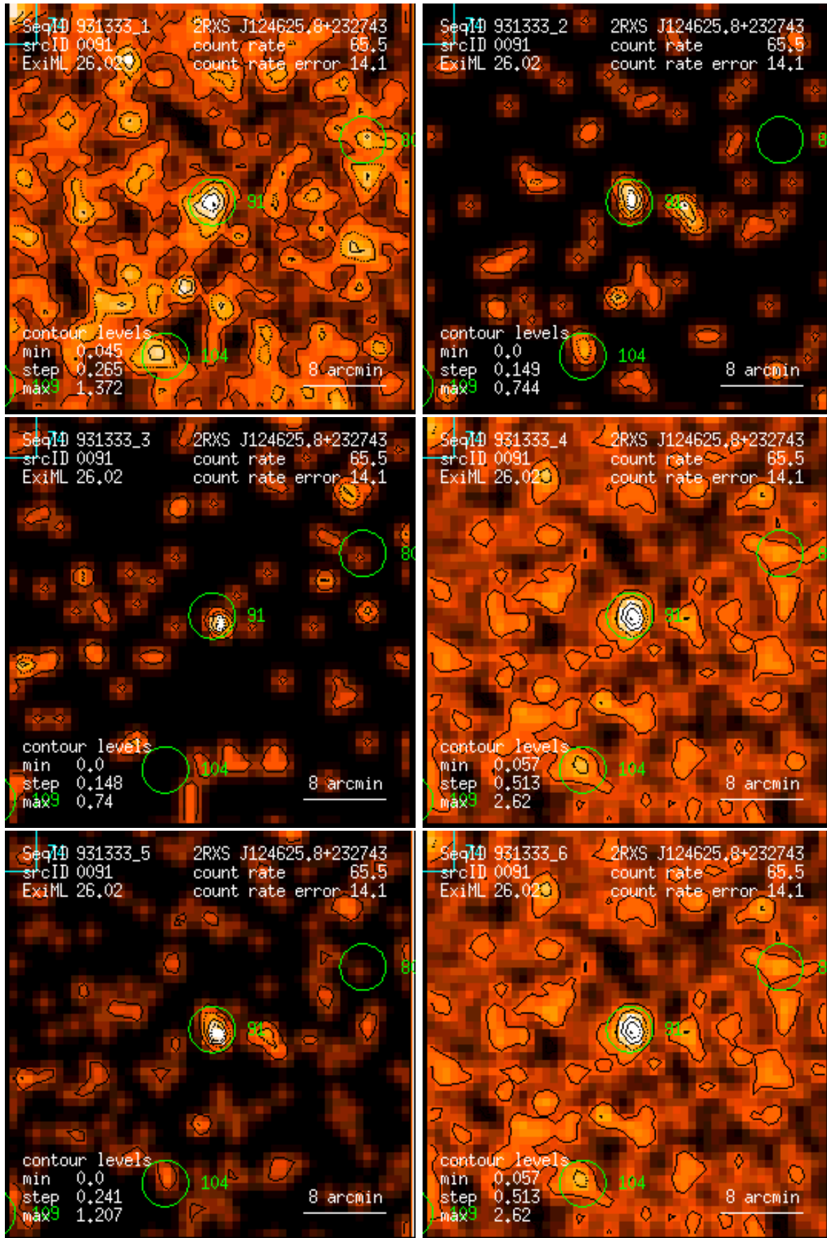
Figure 91: RASS 931333: detection 0091: band rate images, Gaussian filter: (1) PSPC channels 11 – 41, (2) 52 – 90, (3) 91 – 201, (4) 11 – 235, (5) 52 – 201, (6) 11 – 201. Broad band rates in counts/ks. Band rate contour levels in counts/ks/arcmin 2 .
