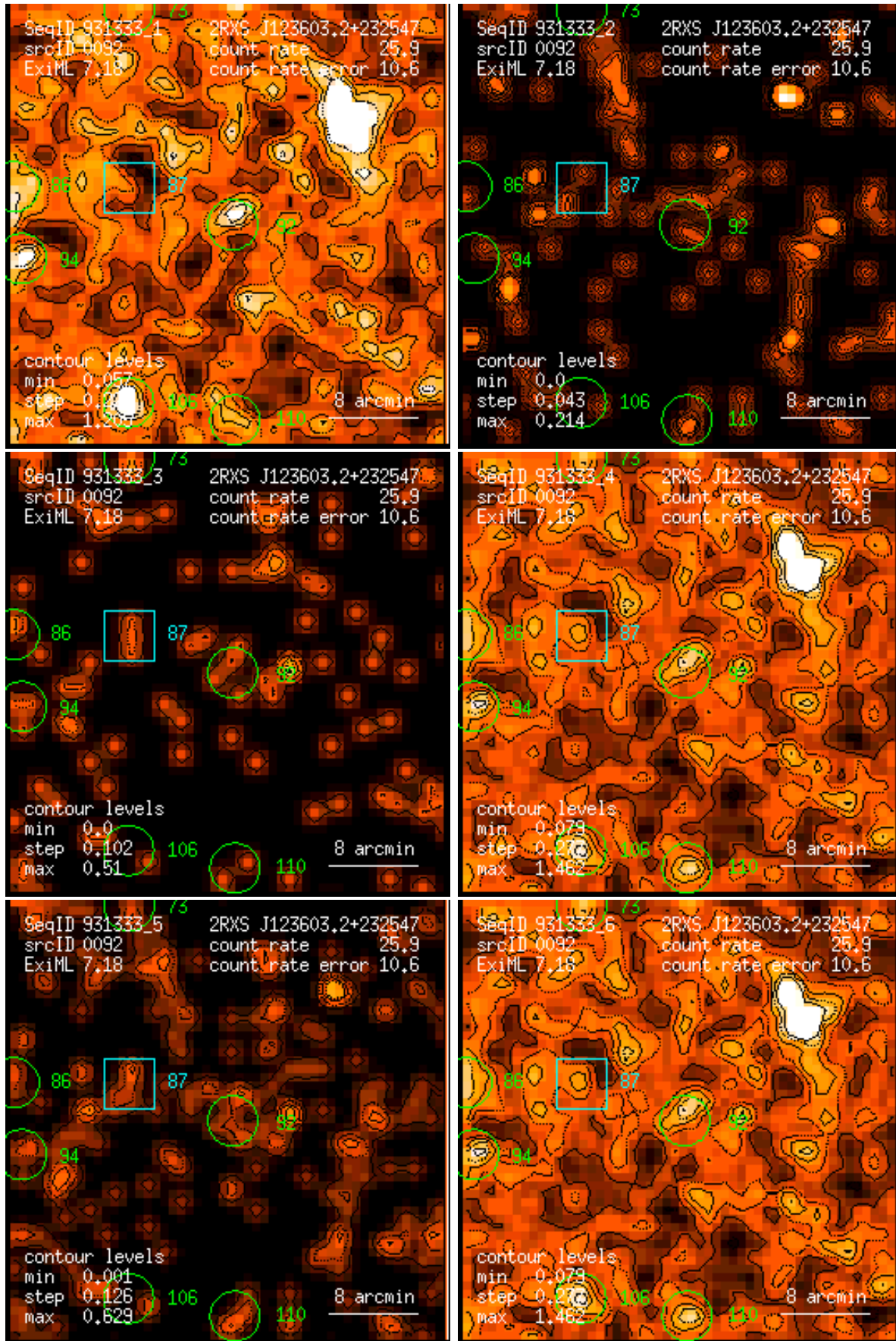
Figure 92: RASS 931333: detection 0092: band rate images, Gaussian filter: (1) PSPC channels 11 – 41, (2) 52 – 90, (3) 91 – 201, (4) 11 – 235, (5) 52 – 201, (6) 11 – 201. Broad band rates in counts/ks. Band rate contour levels in counts/ks/arcmin 2 .
