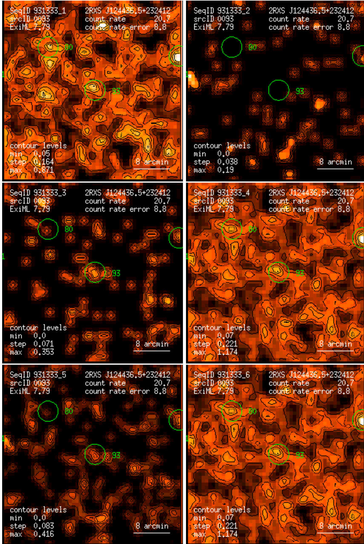
Figure 93: RASS 931333: detection 0093: band rate images, Gaussian filter: (1) PSPC channels 11 – 41, (2) 52 – 90, (3) 91 – 201, (4) 11 – 235, (5) 52 – 201, (6) 11 – 201. Broad band rates in counts/ks. Band rate contour levels in counts/ks/arcmin 2 .
