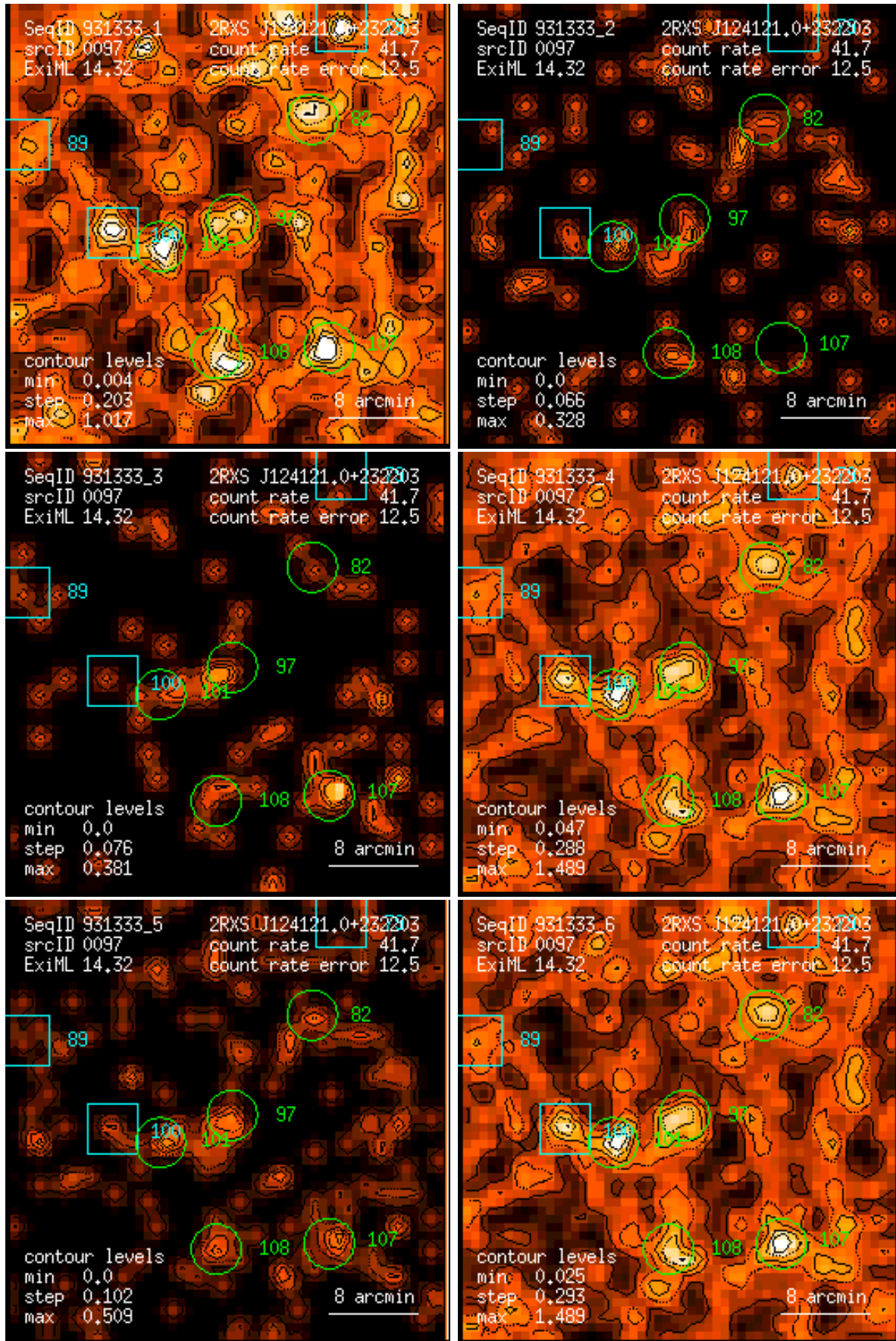
Figure 97: RASS 931333: detection 0097: band rate images, Gaussian filter: (1) PSPC channels 11 – 41, (2) 52 – 90, (3) 91 – 201, (4) 11 – 235, (5) 52 – 201, (6) 11 – 201. Broad band rates in counts/ks. Band rate contour levels in counts/ks/arcmin 2 .
