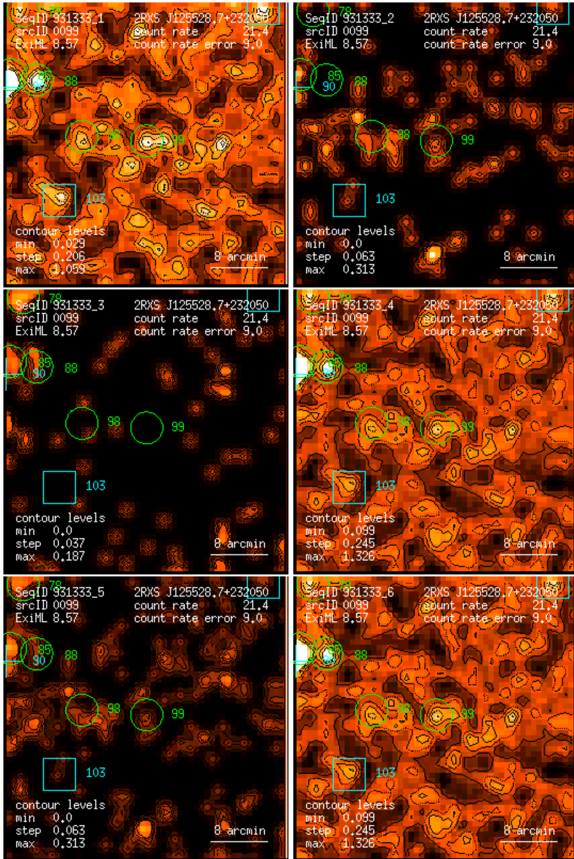
Figure 99: RASS 931333: detection 0099: band rate images, Gaussian filter: (1) PSPC channels 11 – 41, (2) 52 – 90, (3) 91 – 201, (4) 11 – 235, (5) 52 – 201, (6) 11 – 201. Broad band rates in counts/ks. Band rate contour levels in counts/ks/arcmin 2 .
