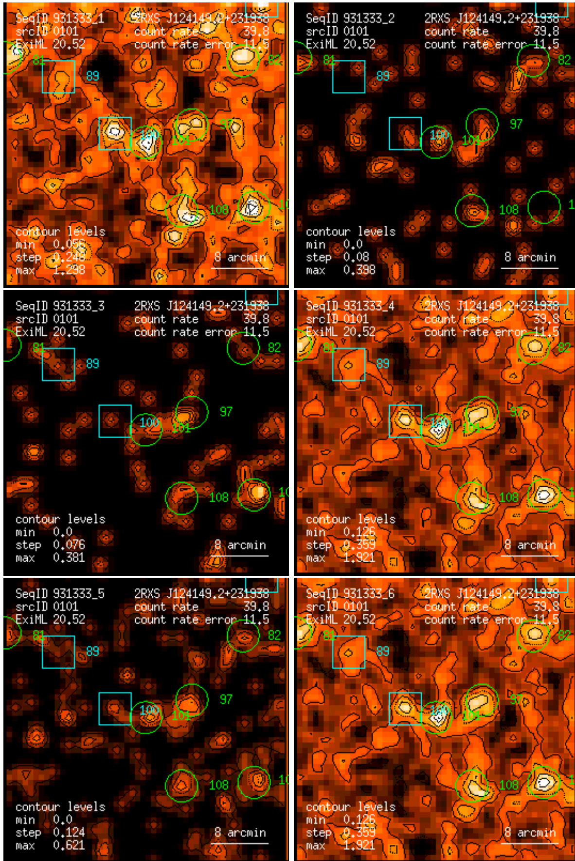
Figure 101: RASS 931333: detection 0101: band rate images, Gaussian filter: (1) PSPC channels 11 – 41, (2) 52 – 90, (3) 91 – 201, (4) 11 – 235, (5) 52 – 201, (6) 11 – 201. Broad band rates in counts/ks. Band rate contour levels in counts/ks/arcmin 2 .
