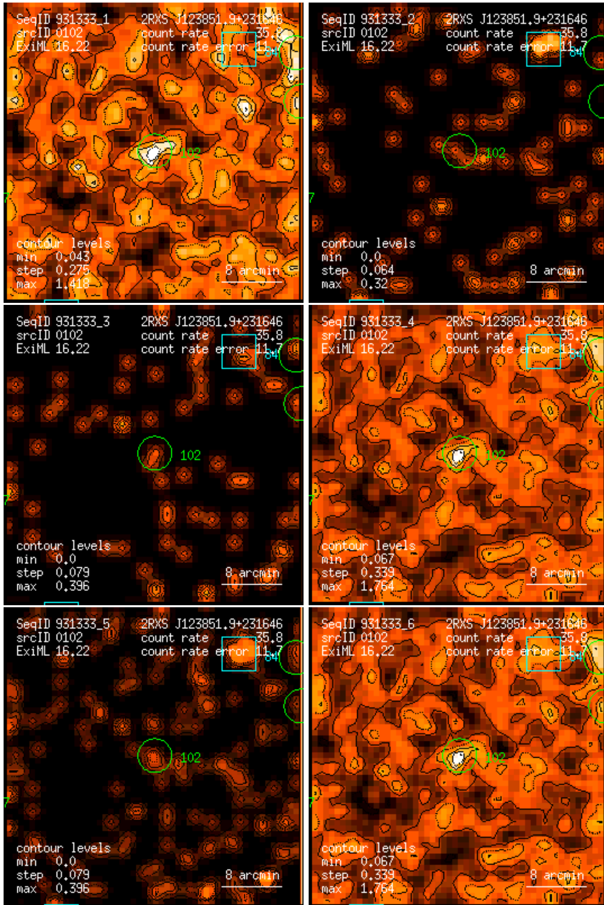
Figure 102: RASS 931333: detection 0102: band rate images, Gaussian filter: (1) PSPC channels 11 – 41, (2) 52 – 90, (3) 91 – 201, (4) 11 – 235, (5) 52 – 201, (6) 11 – 201. Broad band rates in counts/ks. Band rate contour levels in counts/ks/arcmin 2 .
