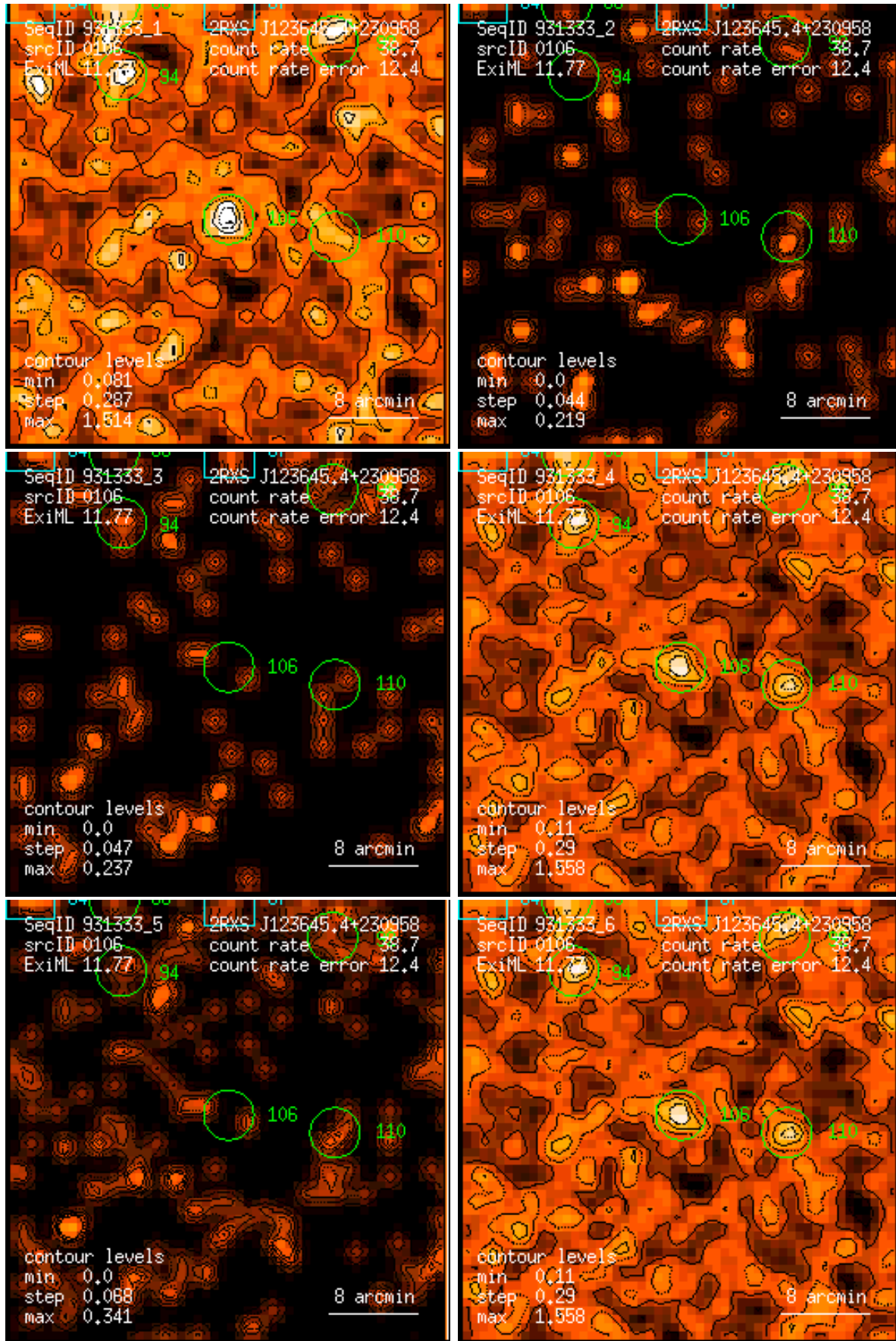
Figure 106: RASS 931333: detection 0106: band rate images, Gaussian filter: (1) PSPC channels 11 – 41, (2) 52 – 90, (3) 91 – 201, (4) 11 – 235, (5) 52 – 201, (6) 11 – 201. Broad band rates in counts/ks. Band rate contour levels in counts/ks/arcmin 2 .
