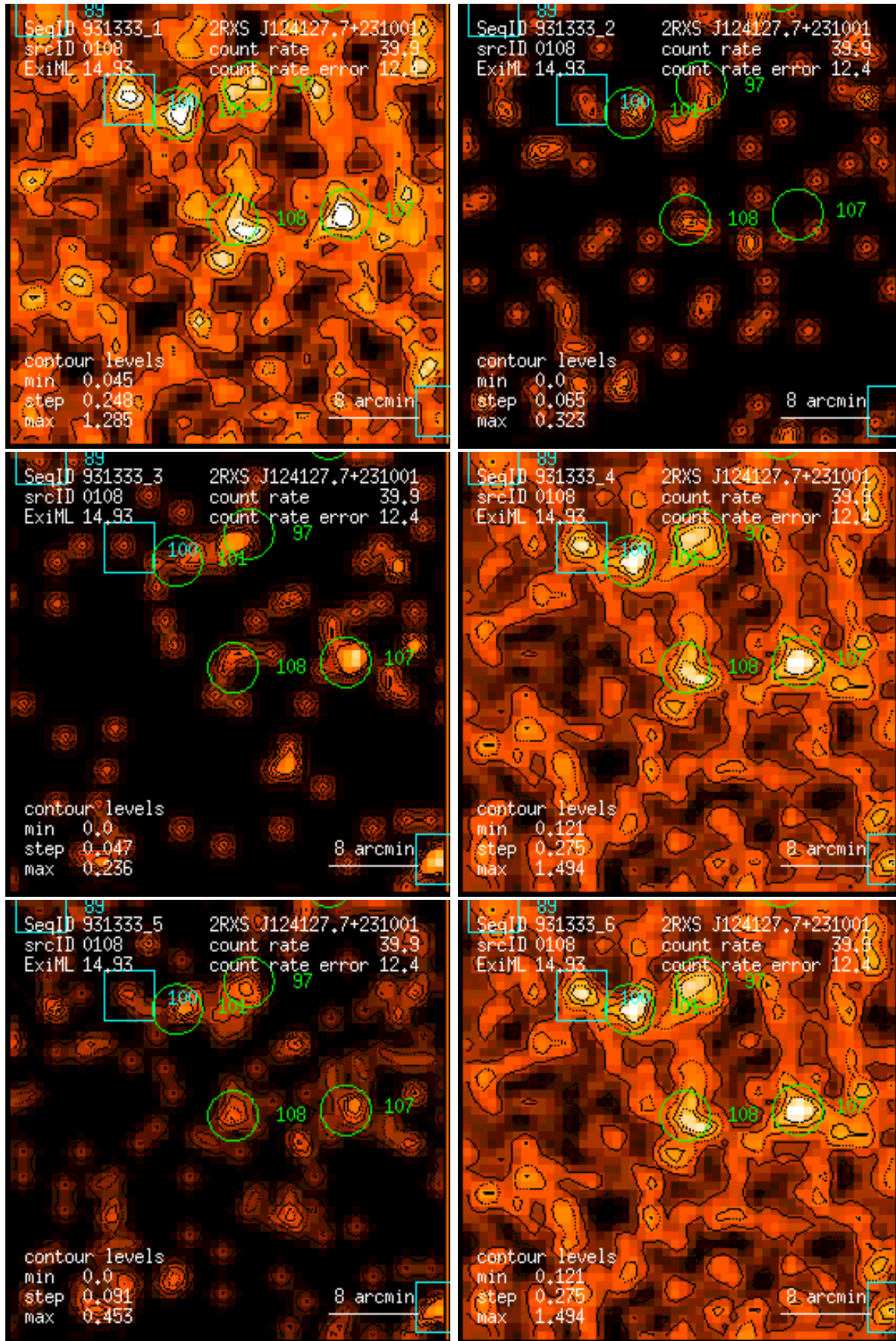
Figure 108: RASS 931333: detection 0108: band rate images, Gaussian filter: (1) PSPC channels 11 – 41, (2) 52 – 90, (3) 91 – 201, (4) 11 – 235, (5) 52 – 201, (6) 11 – 201. Broad band rates in counts/ks. Band rate contour levels in counts/ks/arcmin 2 .
