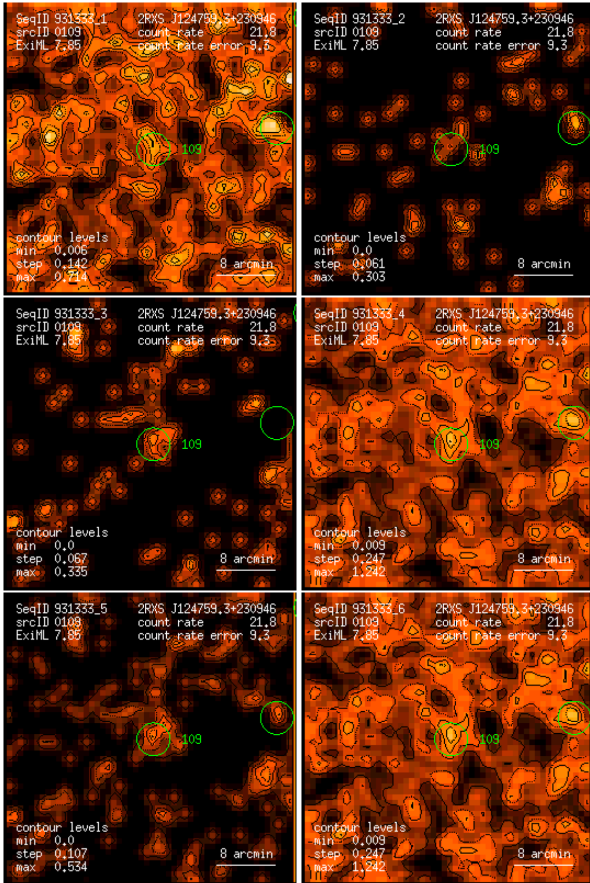
Figure 109: RASS 931333: detection 0109: band rate images, Gaussian filter: (1) PSPC channels 11 – 41, (2) 52 – 90, (3) 91 – 201, (4) 11 – 235, (5) 52 – 201, (6) 11 – 201. Broad band rates in counts/ks. Band rate contour levels in counts/ks/arcmin 2 .
