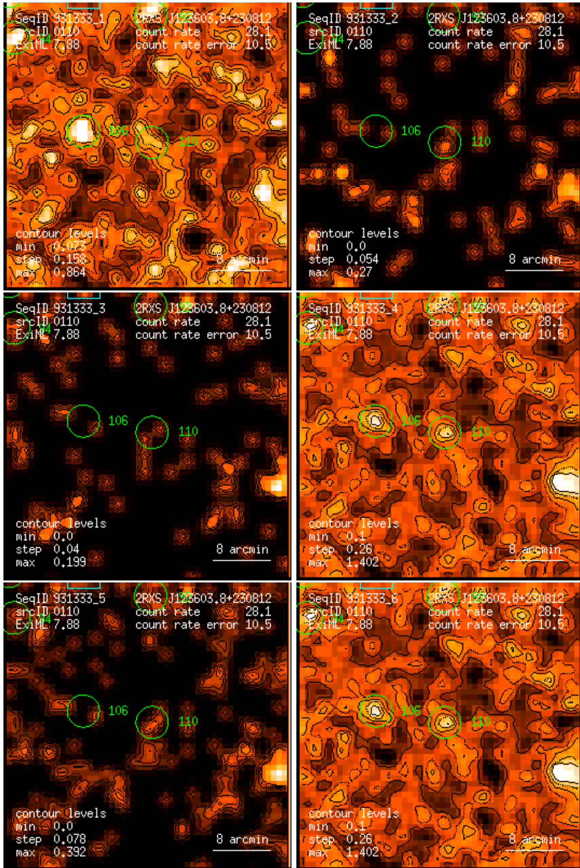
Figure 110: RASS 931333: detection 0110: band rate images, Gaussian filter: (1) PSPC channels 11 – 41, (2) 52 – 90, (3) 91 – 201, (4) 11 – 235, (5) 52 – 201, (6) 11 – 201. Broad band rates in counts/ks. Band rate contour levels in counts/ks/arcmin 2 .
