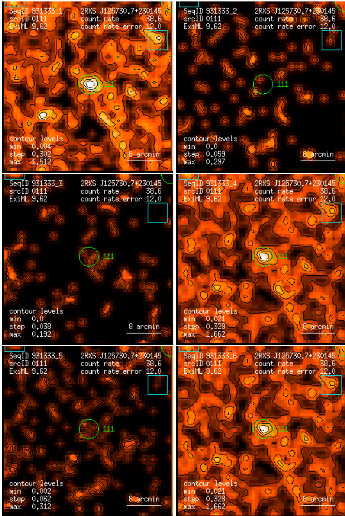
Figure 111: RASS 931333: detection 0111: band rate images, Gaussian filter: (1) PSPC channels 11 – 41, (2) 52 – 90, (3) 91 – 201, (4) 11 – 235, (5) 52 – 201, (6) 11 – 201. Broad band rates in counts/ks. Band rate contour levels in counts/ks/arcmin 2 .
