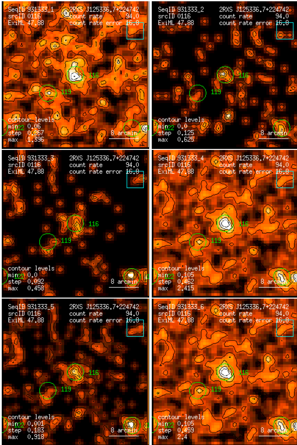
Figure 116: RASS 931333: detection 0116: band rate images, Gaussian filter: (1) PSPC channels 11 – 41, (2) 52 – 90, (3) 91 – 201, (4) 11 – 235, (5) 52 – 201, (6) 11 – 201. Broad band rates in counts/ks. Band rate contour levels in counts/ks/arcmin 2 .
