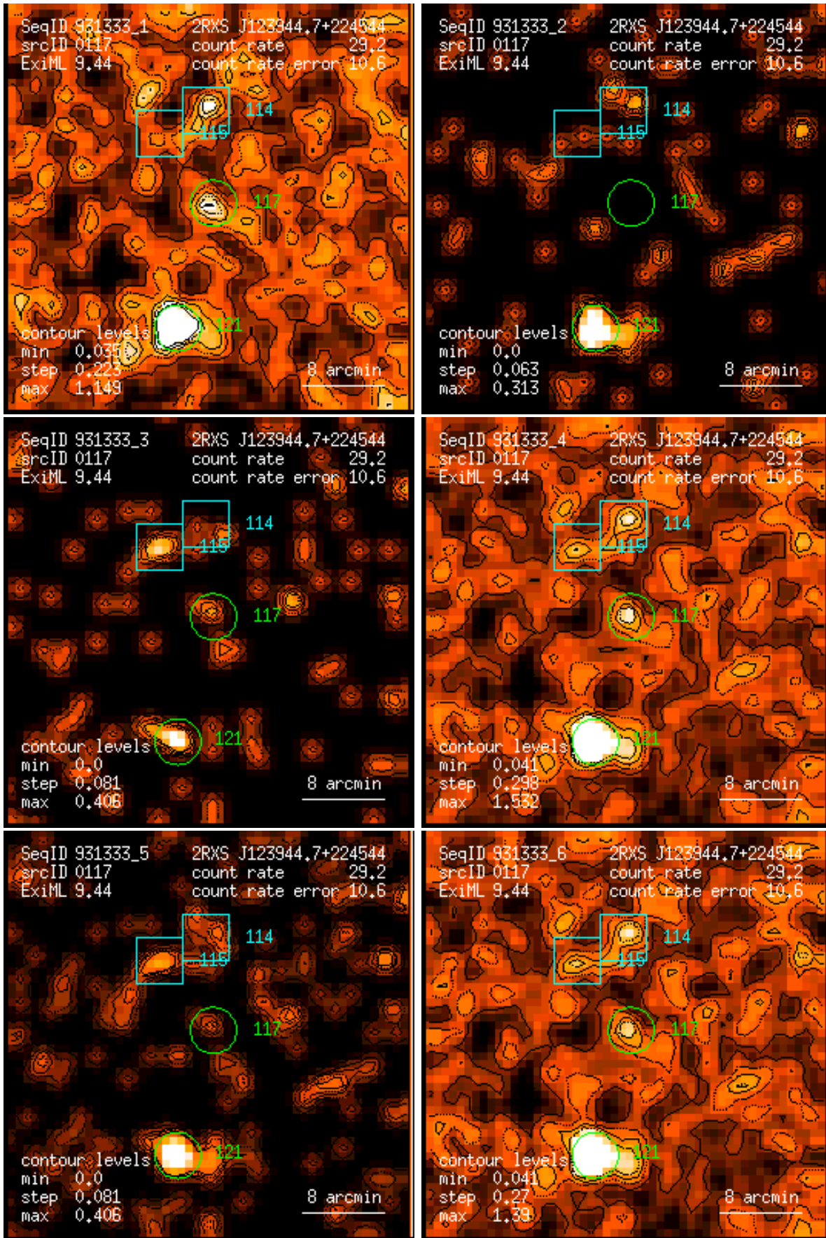
Figure 117: RASS 931333: detection 0117: band rate images, Gaussian filter: (1) PSPC channels 11 – 41, (2) 52 – 90, (3) 91 – 201, (4) 11 – 235, (5) 52 – 201, (6) 11 – 201. Broad band rates in counts/ks. Band rate contour levels in counts/ks/arcmin 2 .
