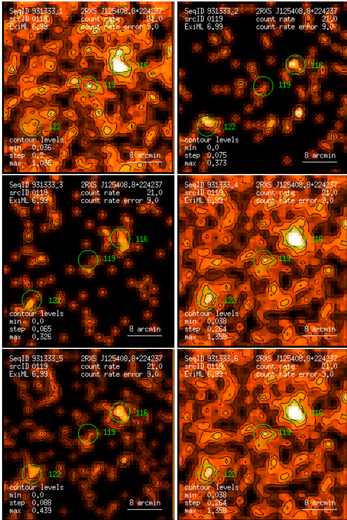
Figure 119: RASS 931333: detection 0119: band rate images, Gaussian filter: (1) PSPC channels 11 – 41, (2) 52 – 90, (3) 91 – 201, (4) 11 – 235, (5) 52 – 201, (6) 11 – 201. Broad band rates in counts/ks. Band rate contour levels in counts/ks/arcmin 2 .
