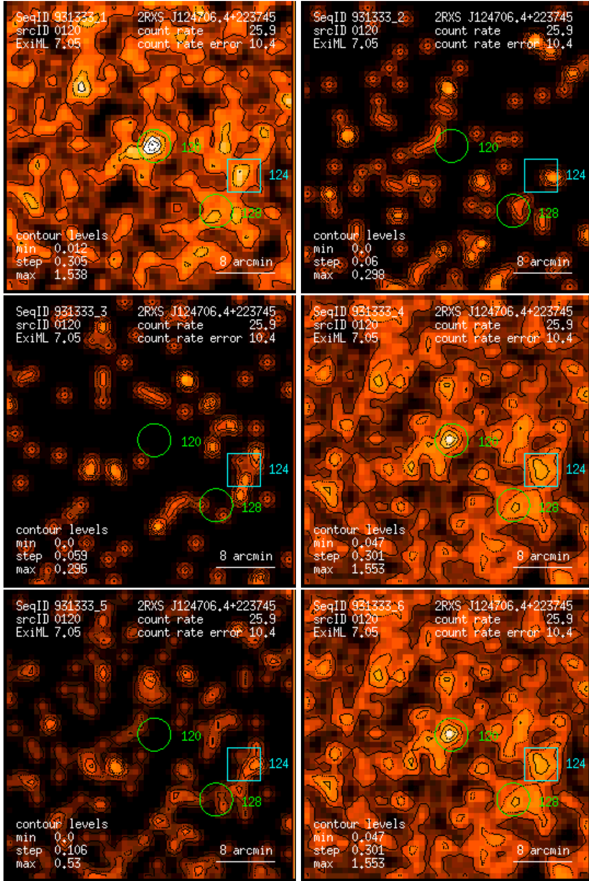
Figure 120: RASS 931333: detection 0120: band rate images, Gaussian filter: (1) PSPC channels 11 – 41, (2) 52 – 90, (3) 91 – 201, (4) 11 – 235, (5) 52 – 201, (6) 11 – 201. Broad band rates in counts/ks. Band rate contour levels in counts/ks/arcmin 2 .
