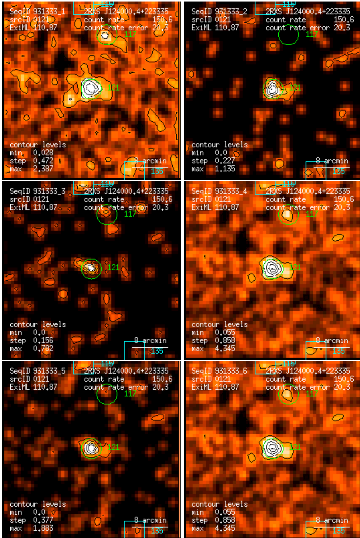
Figure 121: RASS 931333: detection 0121: band rate images, Gaussian filter: (1) PSPC channels 11 – 41, (2) 52 – 90, (3) 91 – 201, (4) 11 – 235, (5) 52 – 201, (6) 11 – 201. Broad band rates in counts/ks. Band rate contour levels in counts/ks/arcmin 2 .
