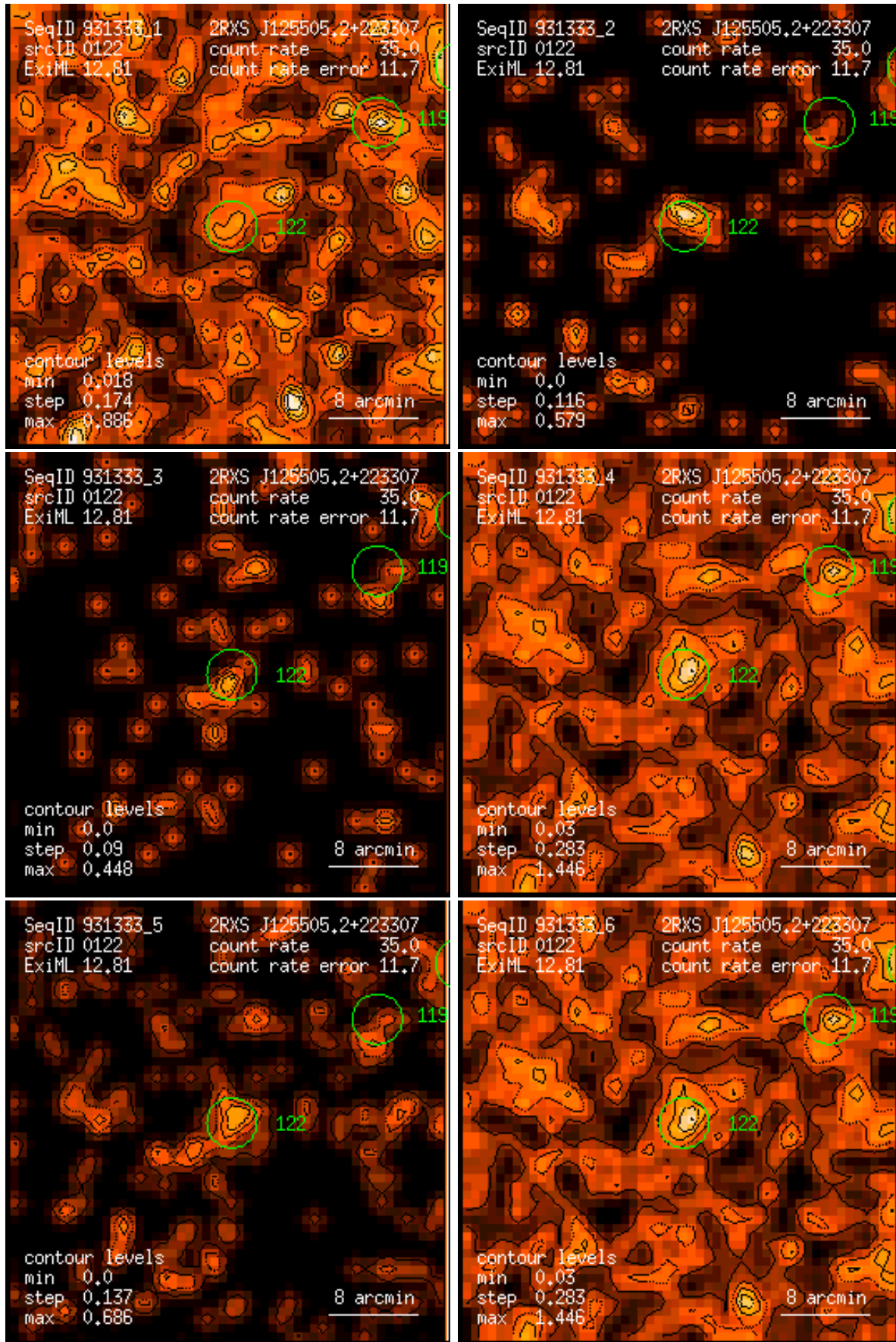
Figure 122: RASS 931333: detection 0122: band rate images, Gaussian filter: (1) PSPC channels 11 – 41, (2) 52 – 90, (3) 91 – 201, (4) 11 – 235, (5) 52 – 201, (6) 11 – 201. Broad band rates in counts/ks. Band rate contour levels in counts/ks/arcmin 2 .
