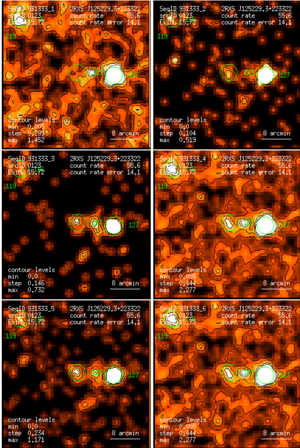
Figure 123: RASS 931333: detection 0123: band rate images, Gaussian filter: (1) PSPC channels 11 – 41, (2) 52 – 90, (3) 91 – 201, (4) 11 – 235, (5) 52 – 201, (6) 11 – 201. Broad band rates in counts/ks. Band rate contour levels in counts/ks/arcmin 2 .
