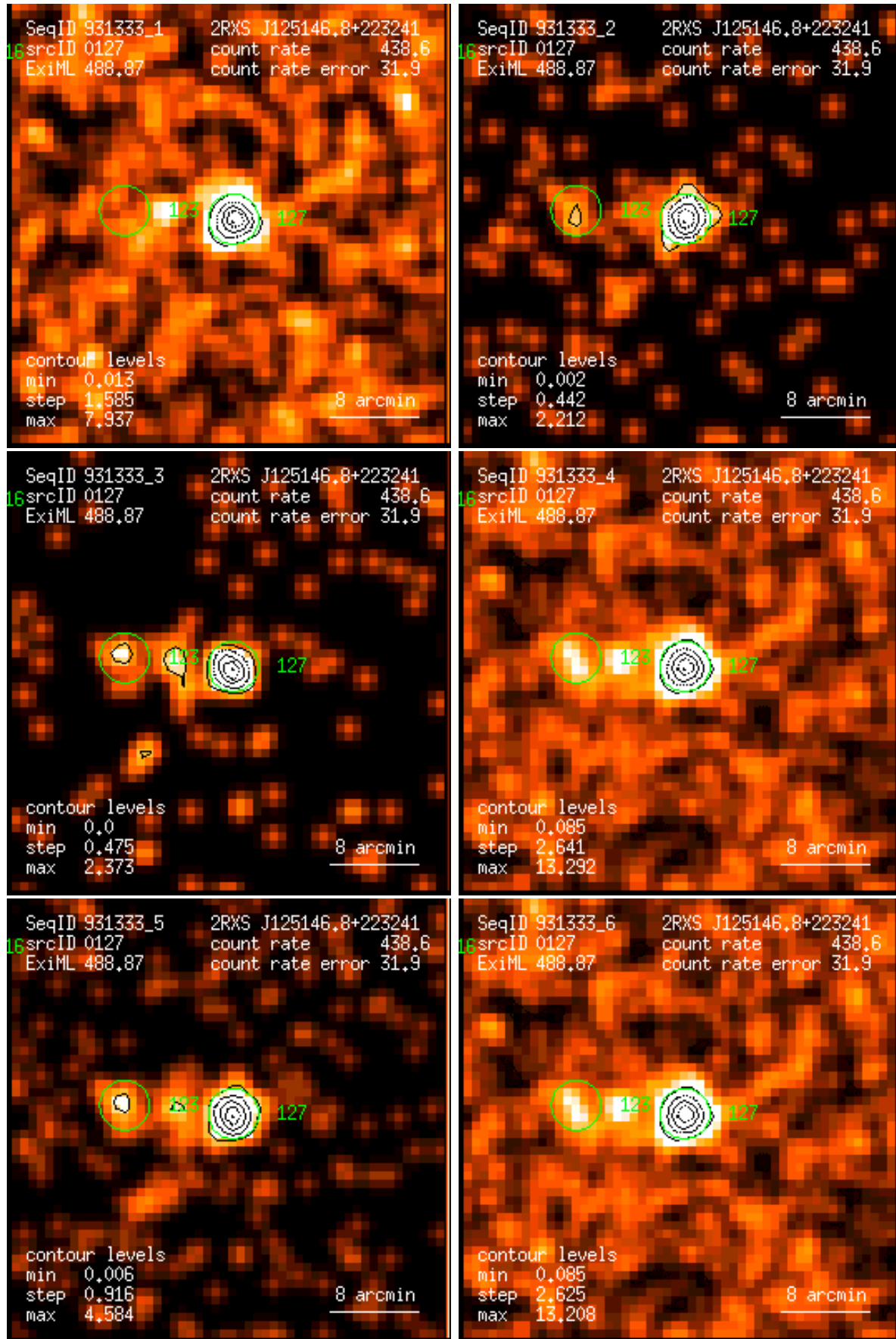
Figure 127: RASS 931333: detection 0127: band rate images, Gaussian filter: (1) PSPC channels 11 – 41, (2) 52 – 90, (3) 91 – 201, (4) 11 – 235, (5) 52 – 201, (6) 11 – 201. Broad band rates in counts/ks. Band rate contour levels in counts/ks/arcmin 2 .
