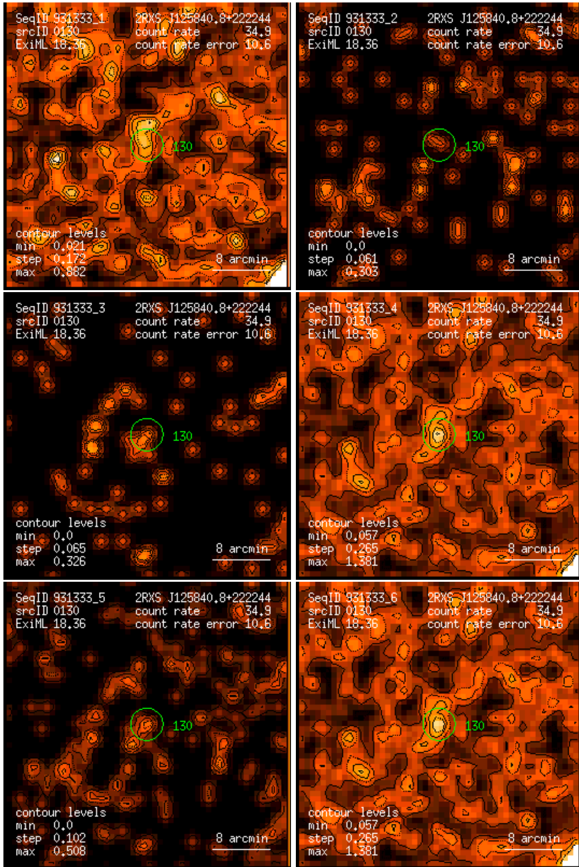
Figure 130: RASS 931333: detection 0130: band rate images, Gaussian filter: (1) PSPC channels 11 – 41, (2) 52 – 90, (3) 91 – 201, (4) 11 – 235, (5) 52 – 201, (6) 11 – 201. Broad band rates in counts/ks. Band rate contour levels in counts/ks/arcmin 2 .
