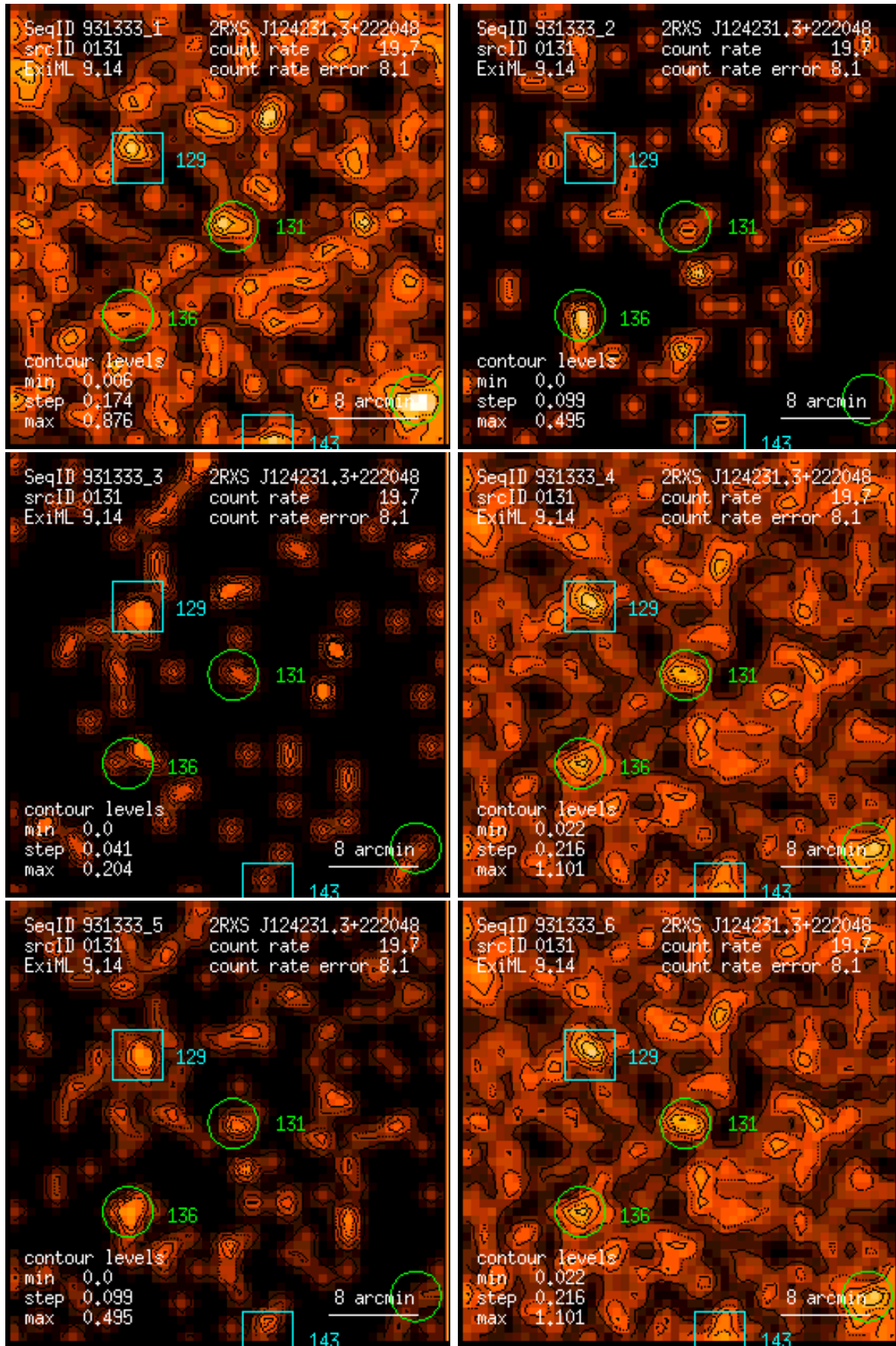
Figure 131: RASS 931333: detection 0131: band rate images, Gaussian filter: (1) PSPC channels 11 – 41, (2) 52 – 90, (3) 91 – 201, (4) 11 – 235, (5) 52 – 201, (6) 11 – 201. Broad band rates in counts/ks. Band rate contour levels in counts/ks/arcmin 2 .
